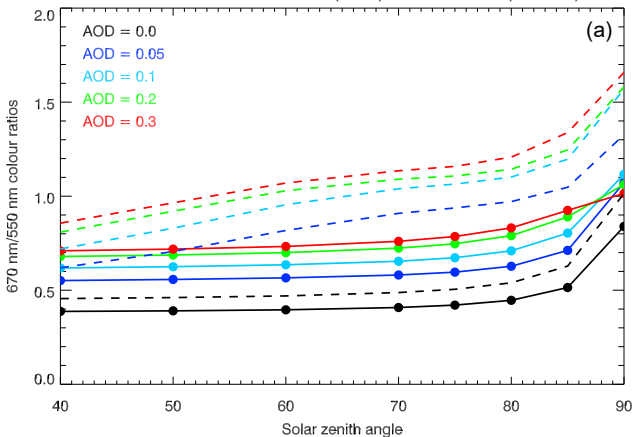
Colour ratios of diffuse flux (solid) and radiance (dashed)
