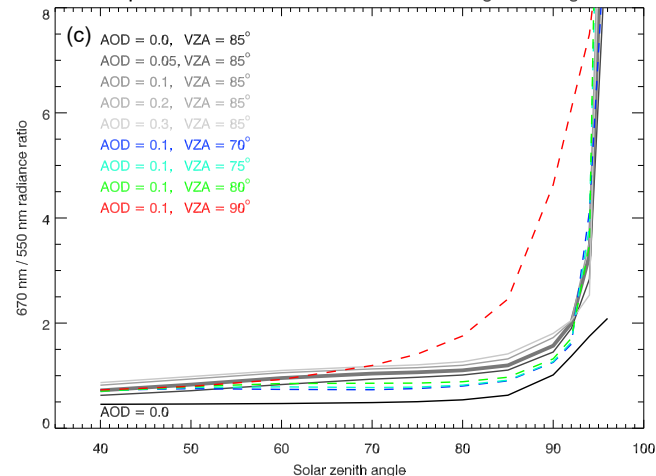
Dependence of 670 nm / 550 nm ratio on viewing zenith angle
