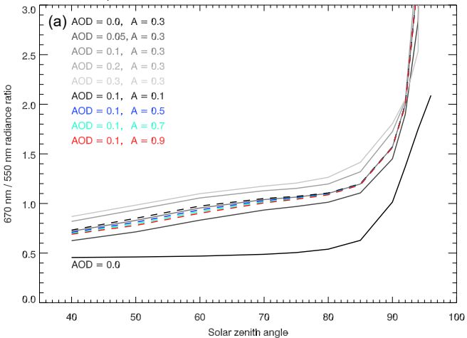
Dependence of 670 nm / 550 nm ratio on surface albedo
