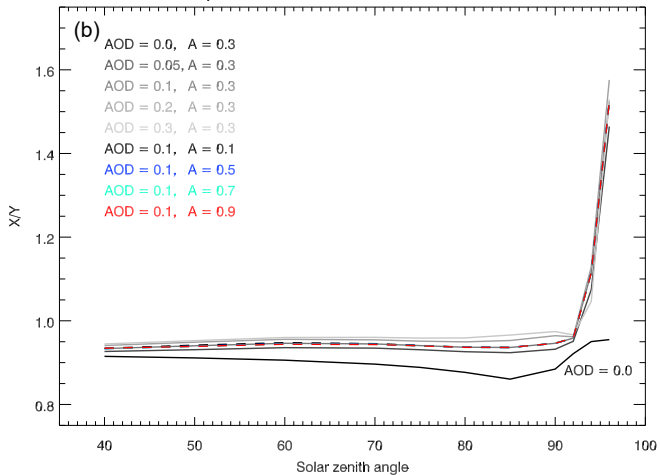
Dependence of X/Y-ratio on surface albedo
