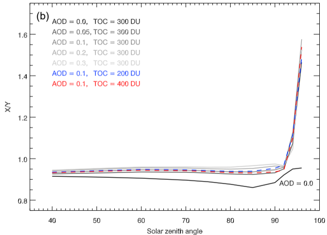
Dependence of X/Y-ratio on total ozone column
