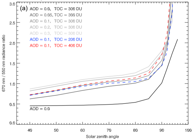
Dependence of 670 nm/550 nm ratio on total ozone column
