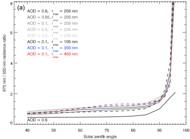
Dependence of 670 nm/550 nm ratio on AOD and particle size
