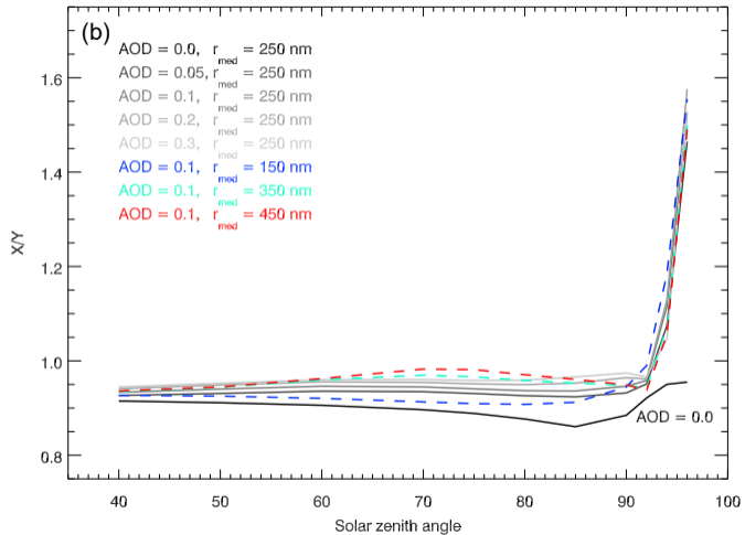
Dependence of X/Y-ratio on AOD and particle size
