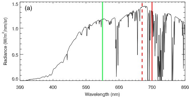
Scattered solar radiation (SZA = 85°, VZA = 85°, SAA = 10°)
