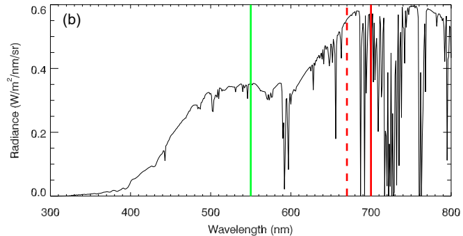
Scattered solar radiation (SZA = 90°, VZA = 85°, SAA = 10°)
