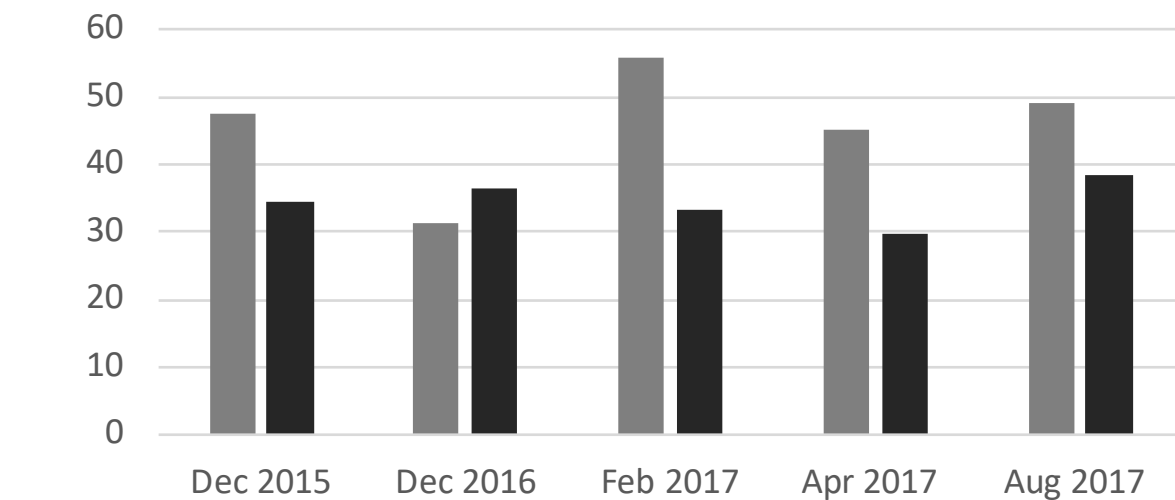
Zr ppm
