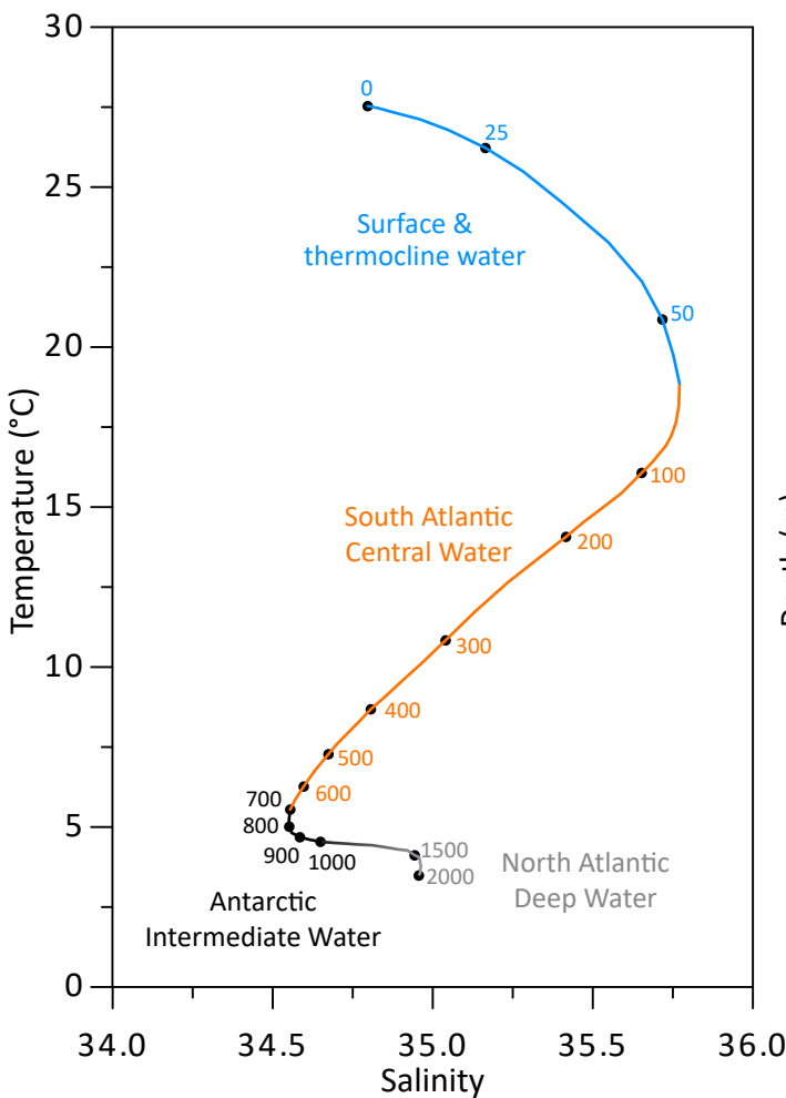
(a) Modern Gulf of Guinea
