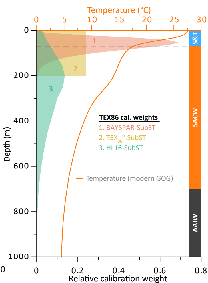
(b) Subsurface calibrations
