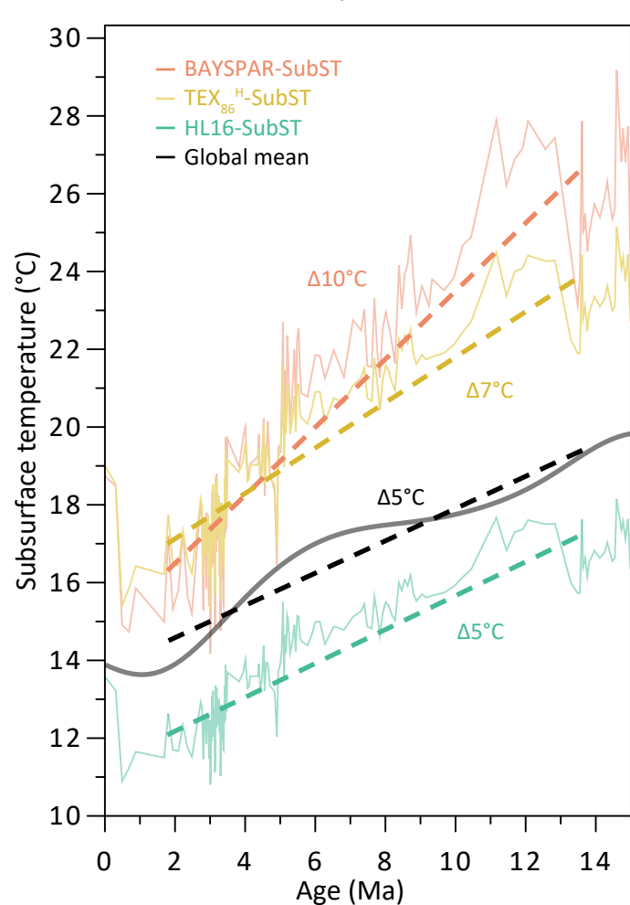
(c) Site 959 temperature evolution
