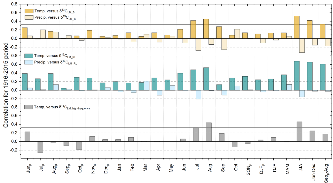
Figure 4. Correlation coefficients between corrected \delta^{13}\text{C}_{\text{LM}_S} , \delta^{13}\text{C}_{\text{LM}_\text{RL}} , \delta^{13}\text{C}_{\text{LM}_\text{high-frequency}} chronologies and local temperatures and precipitation totals from 1916 to 2015. The subscript p indicates the months of the previous year, and horizontal lines indicate the significance levels, with solid lines representing highly significant ( p < 0.001 ) and dashed lines representing significant values ( p < 0.05 ).
