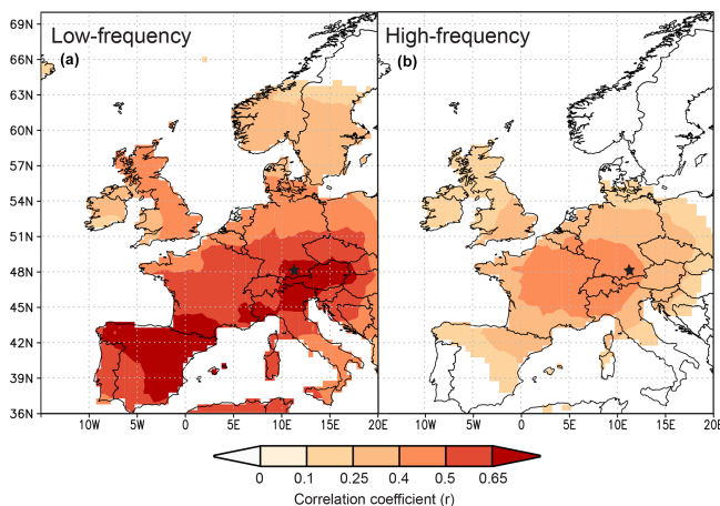
Figure 5. Spatial correlations between summer temperatures (CRU TS4.04) and \delta^{13}\text{C}_{\text{LM}_\text{RL}} anomalies (a) and \delta^{13}\text{C}_{\text{LM}_\text{high-frequency}} indices (b) from 1916–2015. Black star marks the Hohenpeißenberg in Germany.
