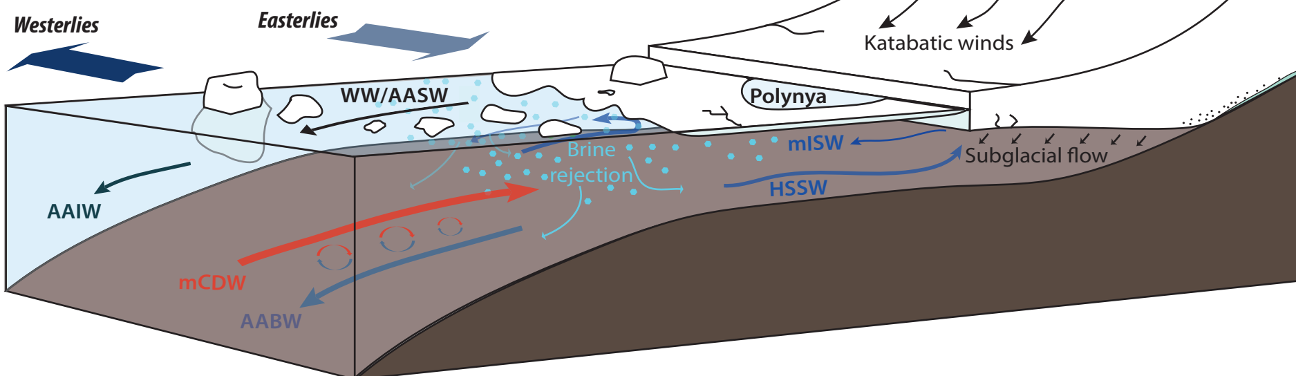
(b) Atmosphere-sea ice
