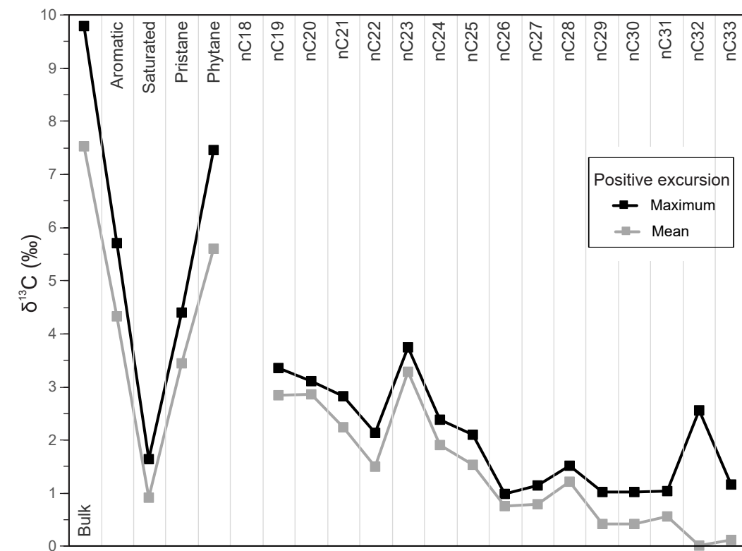
(c) Mean and maximum n -alkane \delta^{13}\text{C} excursion, Taylor White
