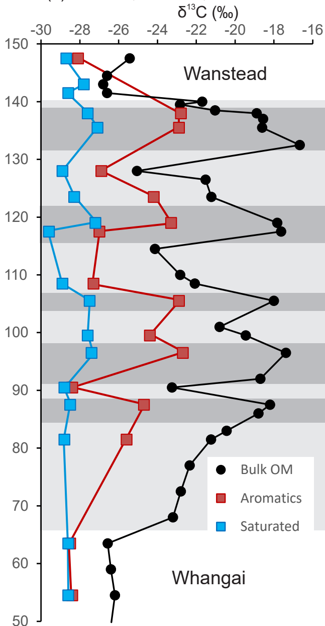
(a) Bulk OM, aromatic, saturated \delta^{13}\text{C}
