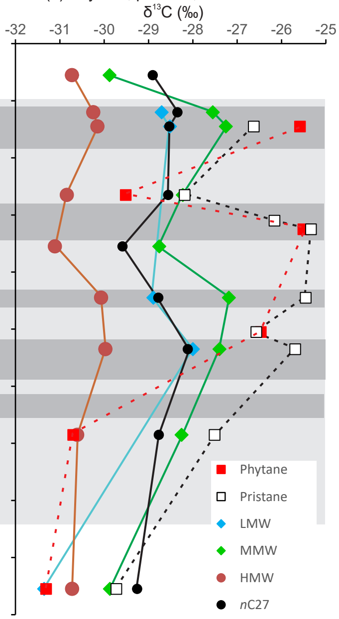
(b) Phytane, pristane, n -alkane \delta^{13}\text{C}
