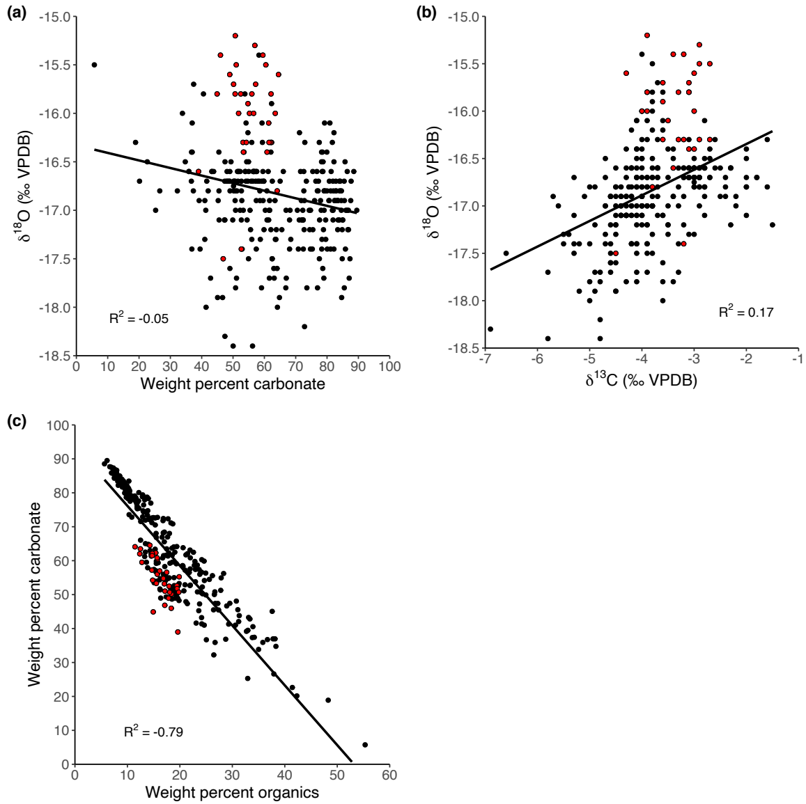
Figure S1. Cross plots of measured isotopic and sediment compositions at Highway 130 Lake (dots) with the linear trends (lines) and coefficients of determination. Samples with ages between 4.2 and 4 ka are colored red.
