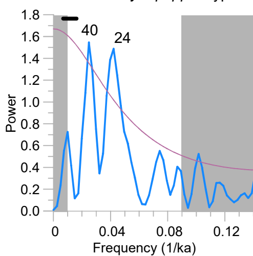
Stoebe-Elytropappus type
