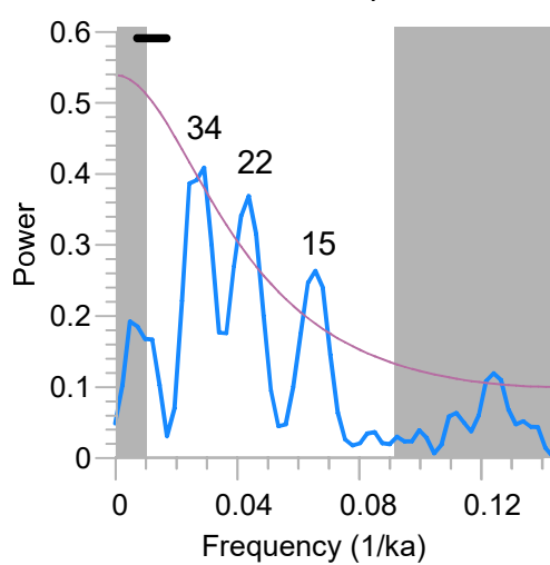
Microcharcoal particles
