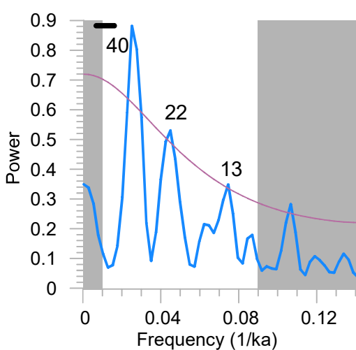
Restionaceae
