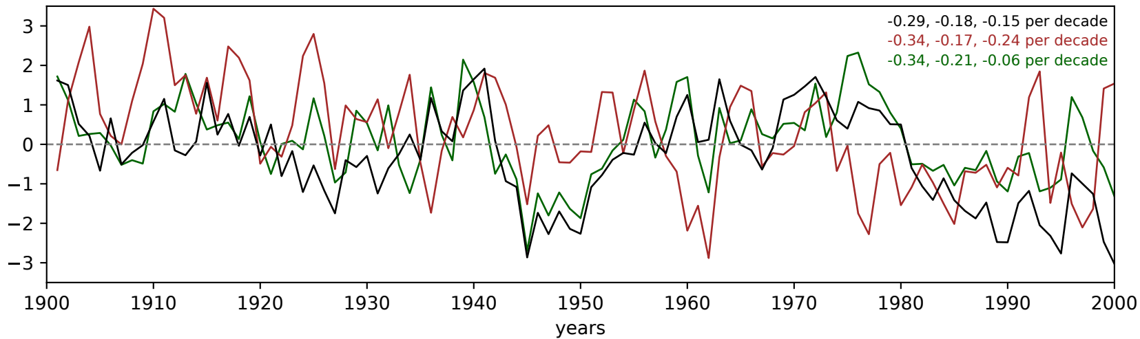
(c) scPDSI Summer
