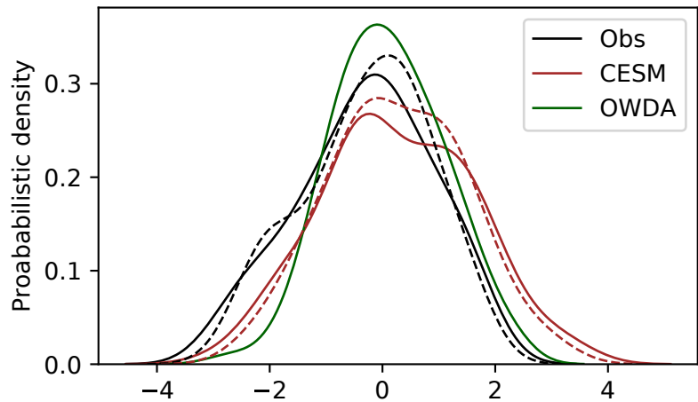
(a) scPDSI Probability Distribution
