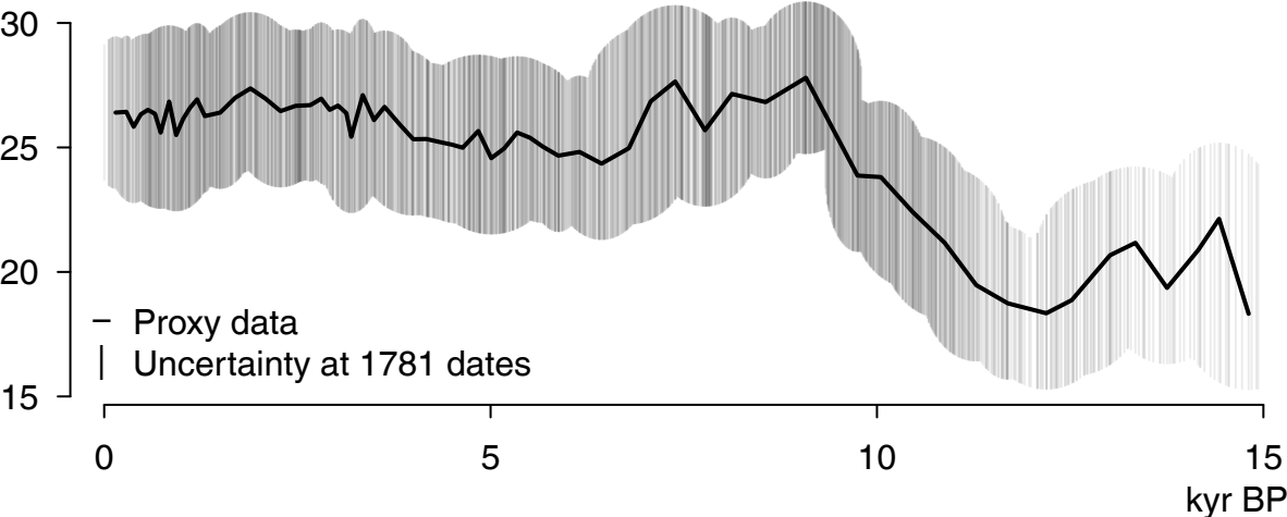
(a) Proxy data in Temperature /°C
