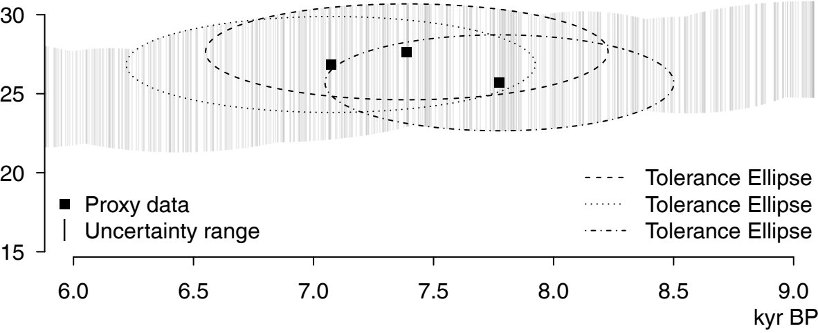
(b) Proxy data in Temperature /°C
