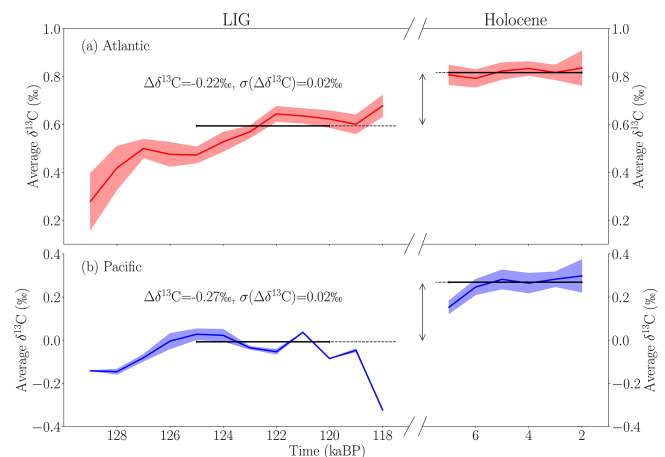
Figure 6. Comparison of volume-weighted \delta^{13}\text{C} for the Atlantic (red) and Pacific (blue) for the LIG and Holocene, calculated using the regions from Peterson et al. (2014) from data covering all depths. Solid coloured lines indicate the mean volume-weighted \delta^{13}\text{C} , and the shading indicates the volume-weighted sum of square deviations from the mean. The horizontal bars indicate the mean of the stable period determined from the regional analysis as defined in Sect. 3.1 (LIG: 125–120 ka BP; Holocene: 7–2 ka BP), with the \Delta\delta^{13}\text{C} indicating the mean anomaly between these two averages and the standard deviation ( \sigma(\delta^{13}\text{C}) , ‰).
