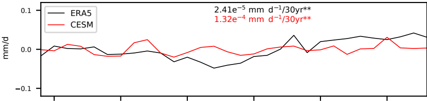
(b) Land annual mean of daily precipitation anomaly
