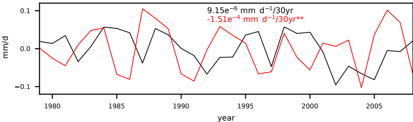
(b) Land annual mean of daily precipitation anomaly
