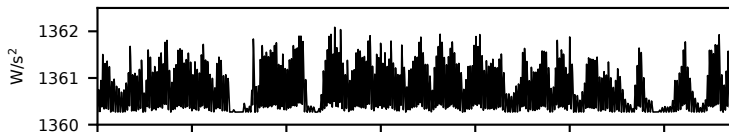
Global Annual Mean Insolation (INS)
