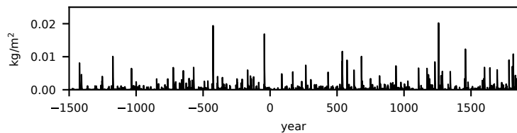
Total Sulfate Aerosol Column Mass (VOL)
