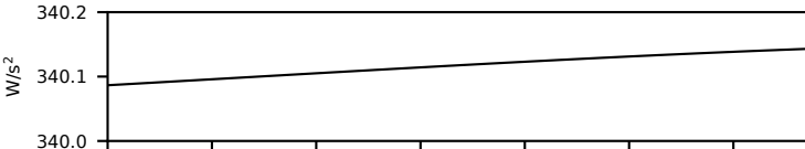
Global Annual Mean Clear Sky Net Surface Shortwave Radiation (FSN)
