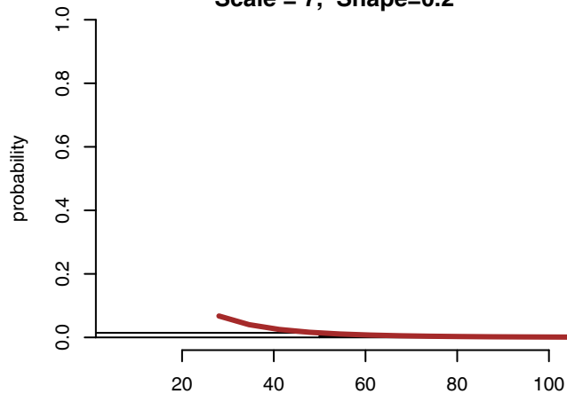
(a) I- High scale, positive shape Scale = 7, Shape=0.2
