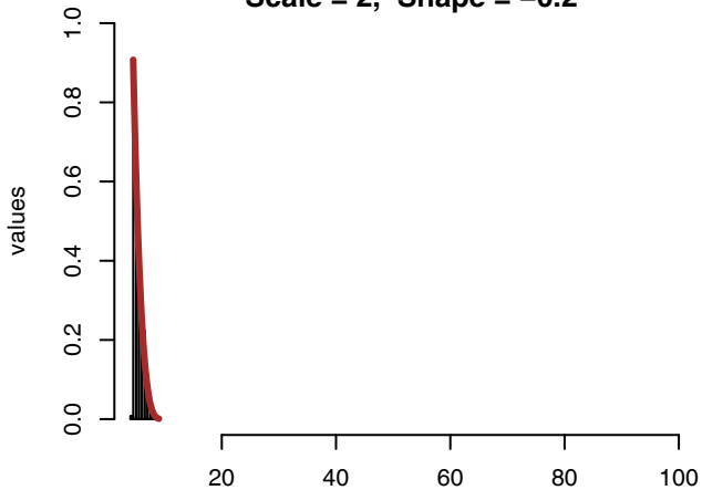
(d) IV- Low scale, negative shape Scale = 2, Shape = -0.2
