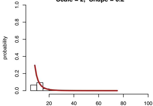
(c) III- Low scale, positive shape Scale = 2, Shape = 0.2
