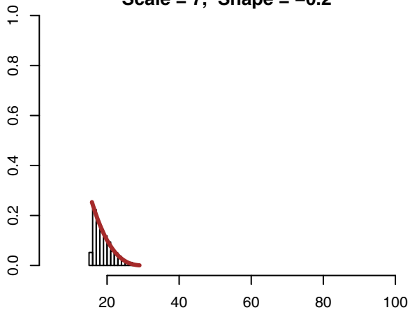
(b) II- High scale, negative shape Scale = 7, Shape = -0.2
