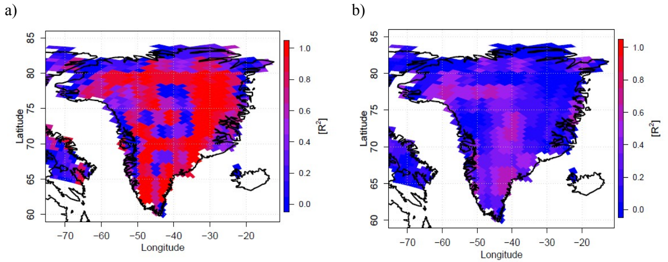
Figure S1: Present-day (period 2008-2014) (a) spatial and (b) temporal \delta^{18}\text{O} -temperature correlation ( R^2 value) for Greenland for COSMO_iso_50km. The temperature correlations are based on yearly mean values.
