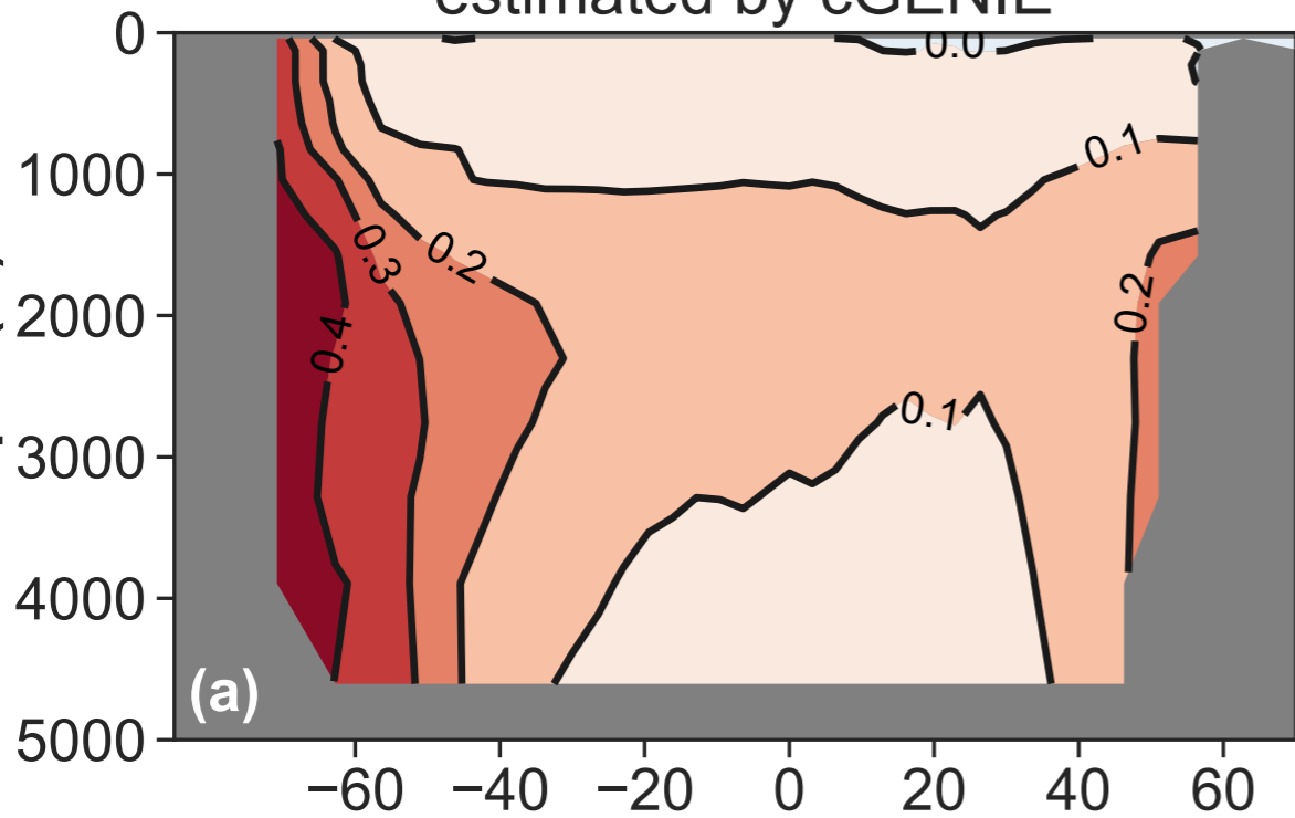
\Delta\delta^{13}\text{C}_{\text{soft}} error (‰) estimated by cGENIE
