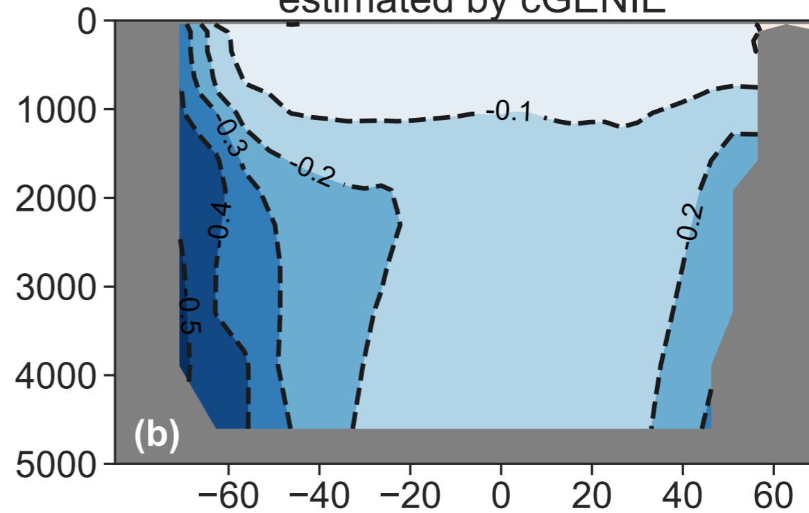
\Delta\delta^{13}\text{C}_{\text{pref}} error (‰) estimated by cGENIE
