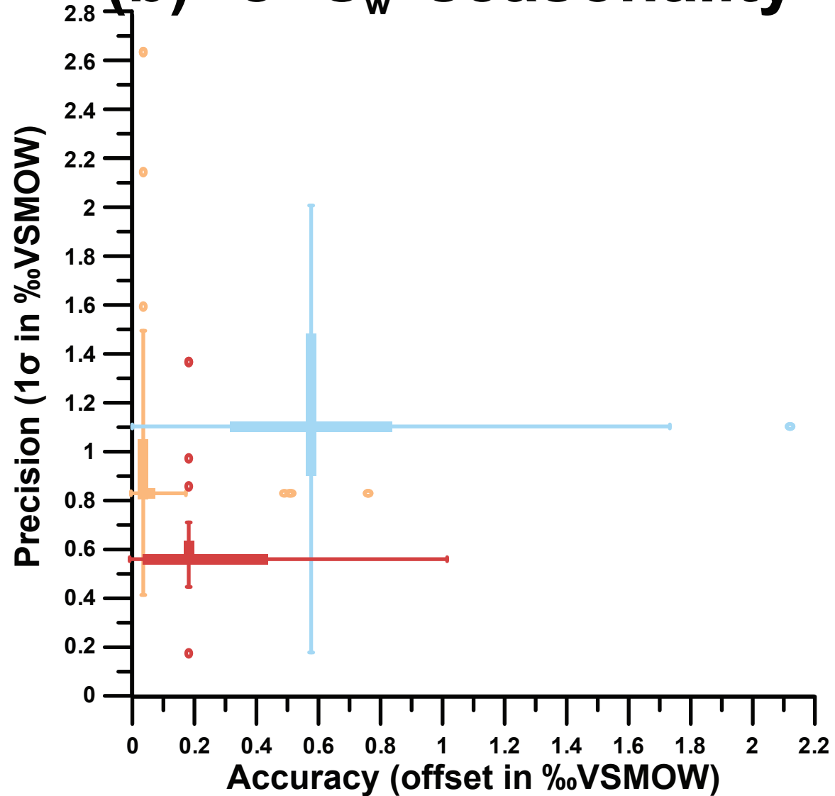
(b) \delta^{18}\text{O}_w seasonality
