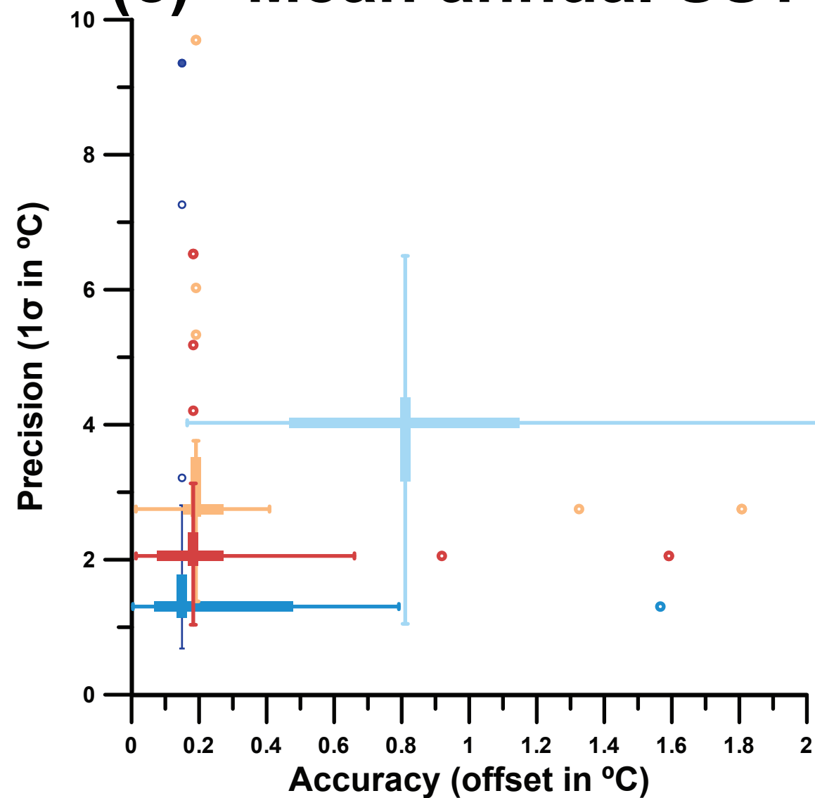
(c) Mean annual SST
