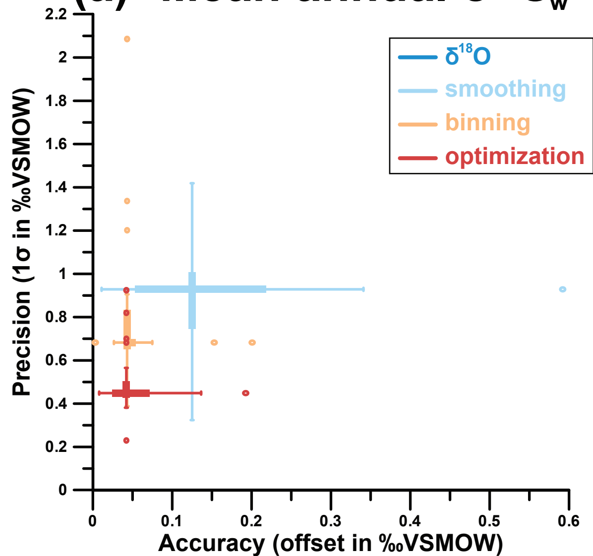
(a) Mean annual \delta^{18}\text{O}_w
