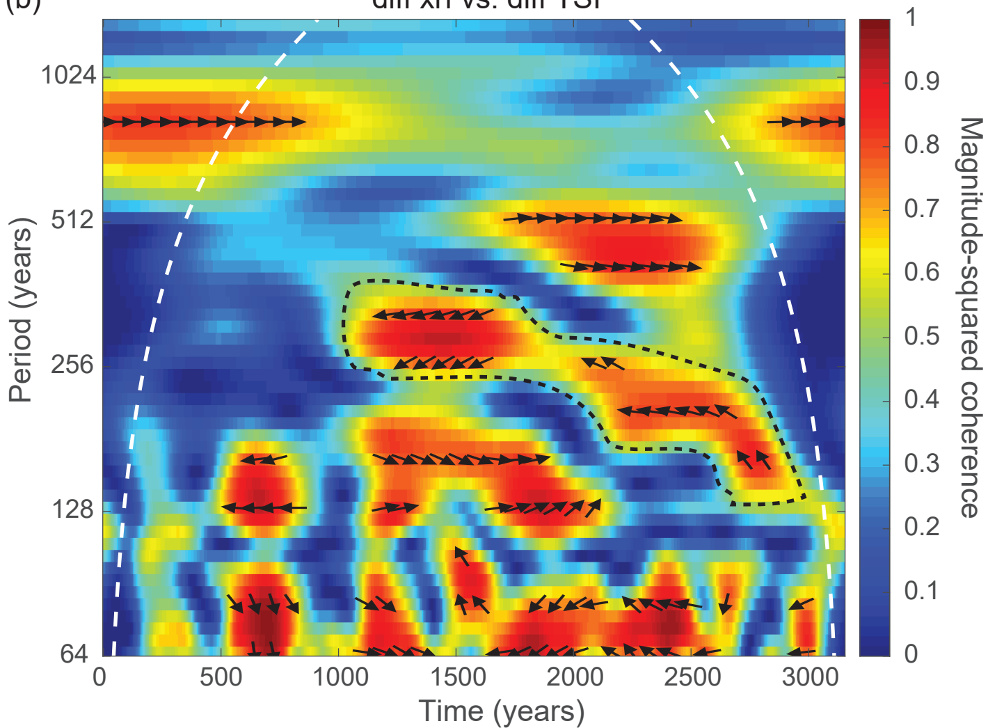
(b) diff xrf vs. diff TSI
