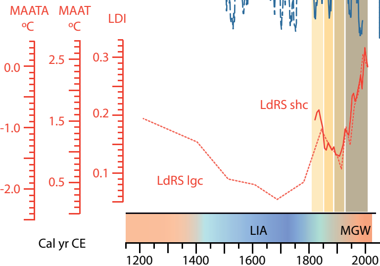
(c) LdRS LDI record
