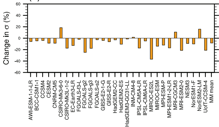
(c) lig127k
