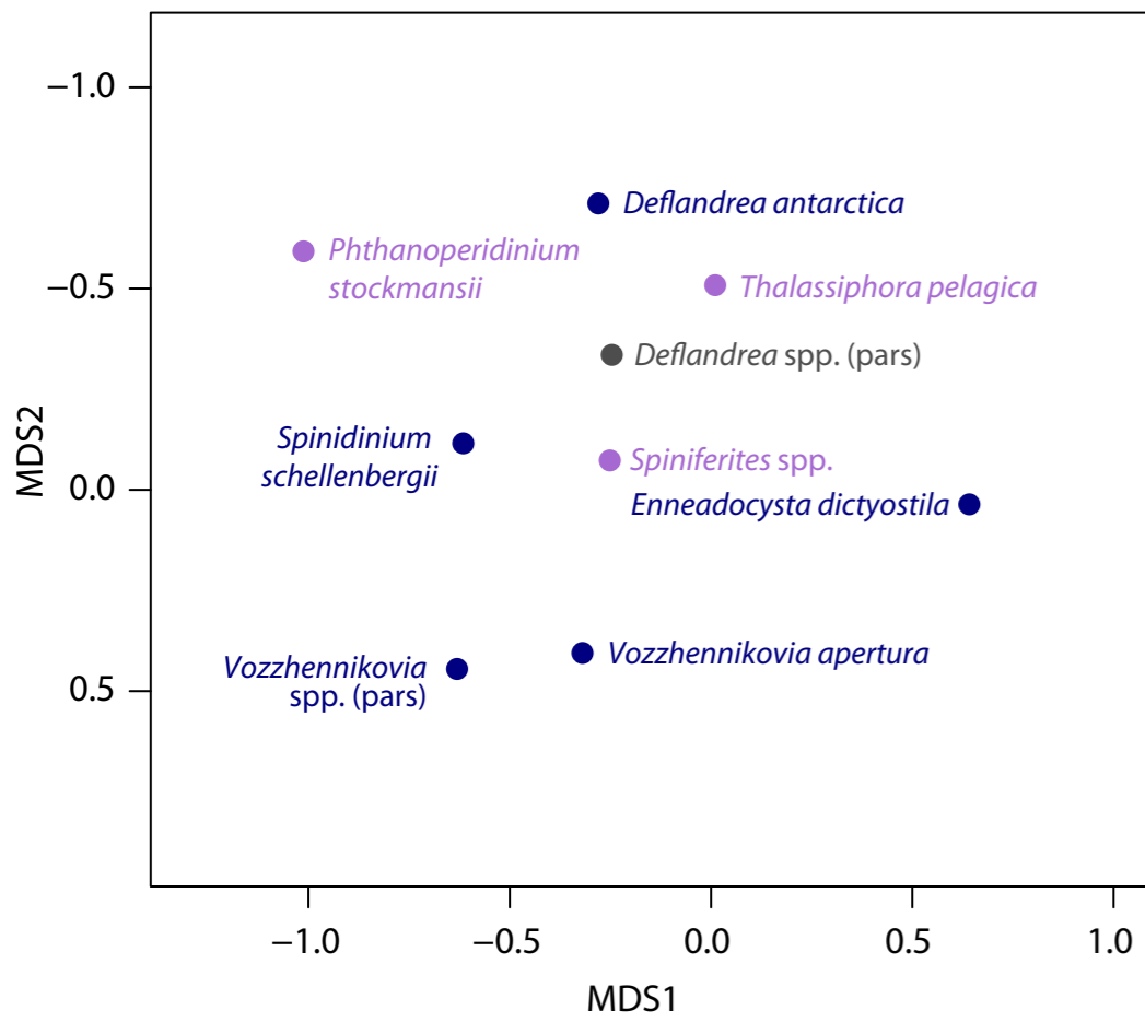
(a) NMDS Site 1170
