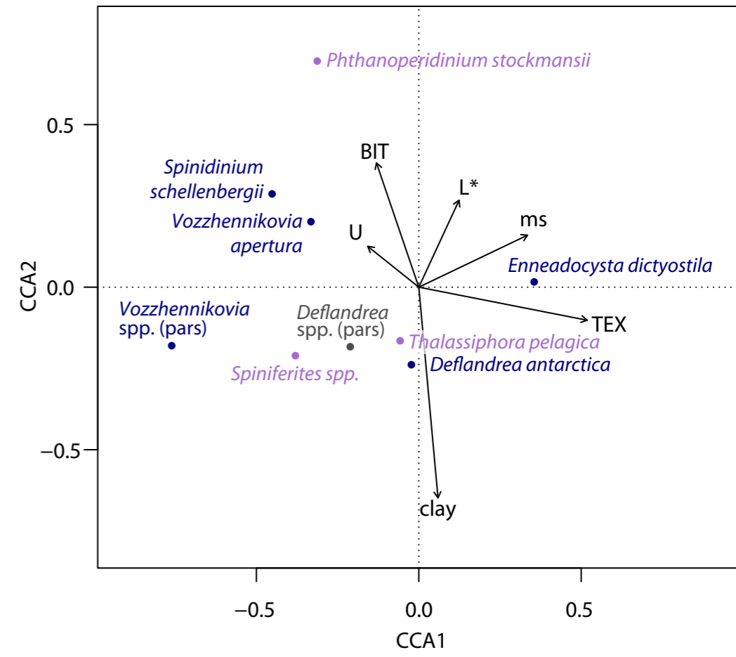
(c) CCA Site 1170
