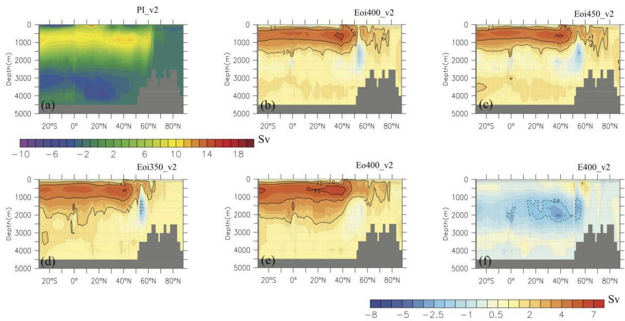
Figure S4: Mean annual AMOC of PI control experiment in IPSLCM5A2 (a) and AMOC anomalies of Eoi400_v2 (b), Eoi450_v2 (c), Eoi350_v2 (d), Eo400_v2 (e) and E400_v2 (f) in comparison with PI condition.
