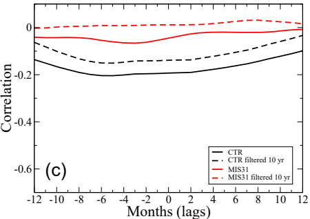
CORRELATION NINO34 and monsoonal precipitation index - EA
