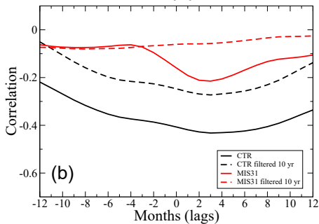
CORRELATION NINO34 and monsoonal precipitation index - WNP
