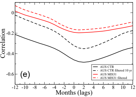
CORRELATION NINO34 and monsoonal precipitation index - AUS
