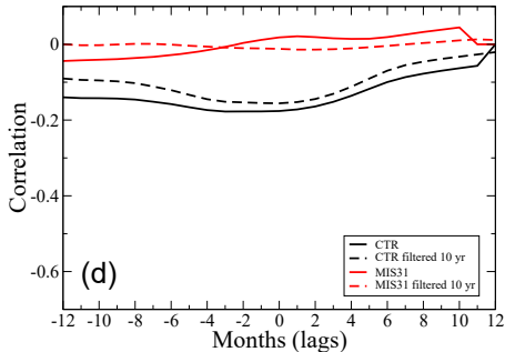
CORRELATION NINO34 and monsoonal precipitation index - IN
