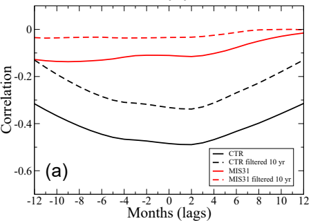
CORRELATION NINO34 and monsoonal precipitation index - AM
