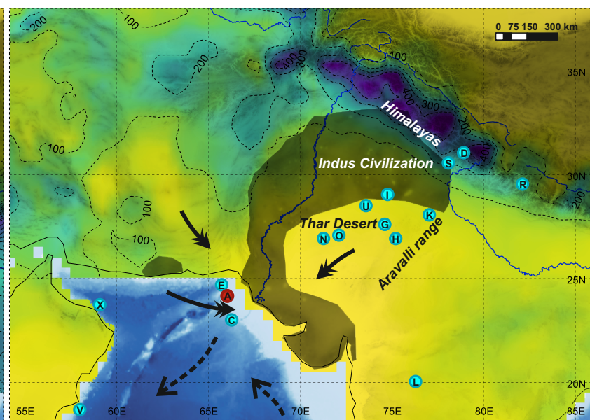
(c) Long-term mean (1981–2010) winter precipitation
