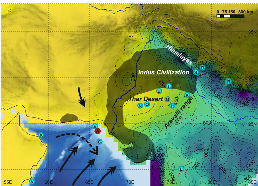
(b) Long-term mean (1981–2010) summer precipitation
