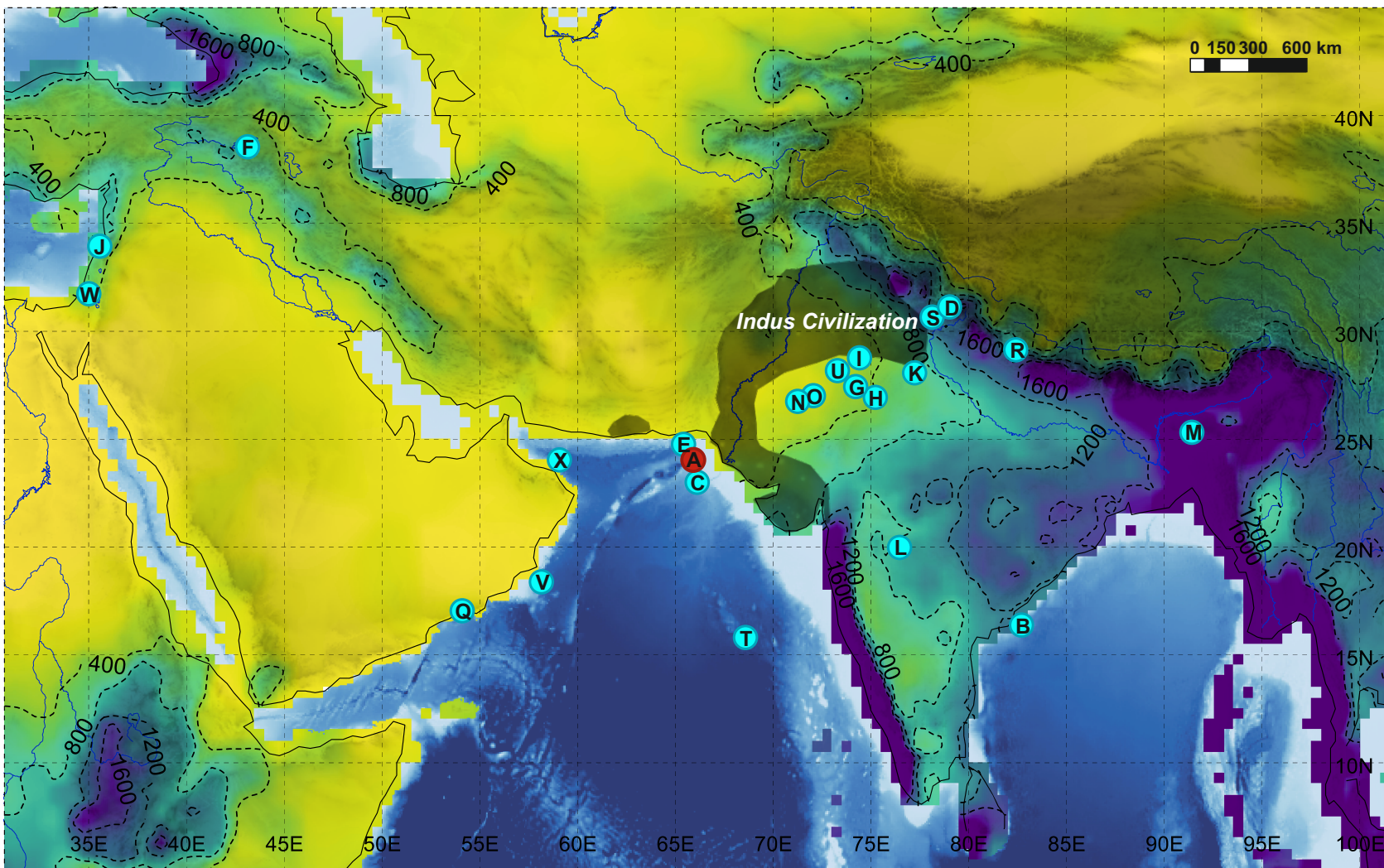
(a) Long-term mean (1981–2010) annual precipitation
