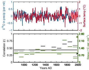
7. DML coast
