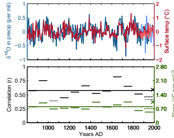
8. West Antarctica
