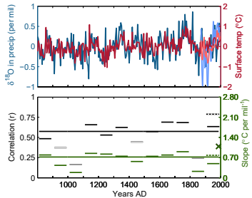
10. Antarctica
