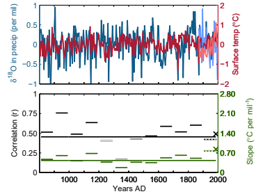
9. East Antarctica
