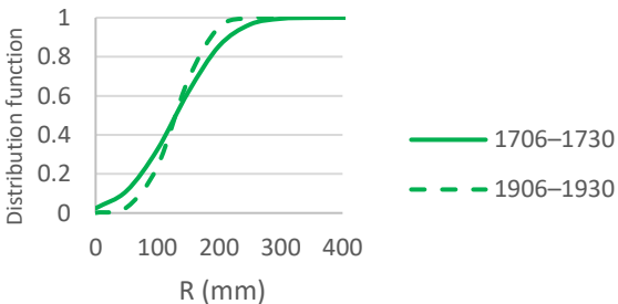
(c) 1706–1730 vs. 1906–1930, spring
