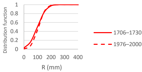
(f) 1706 1730 vs. 1976 2000, autumn
