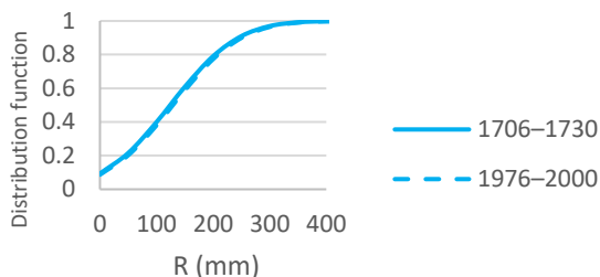
(b) 1706 1730 vs. 1976 2000, winter
