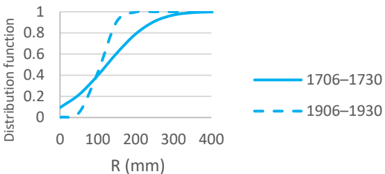
(a) 1706–1730 vs. 1906–1930, winter
