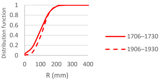
(e) 1706 1730 vs. 1906 1930, autumn
