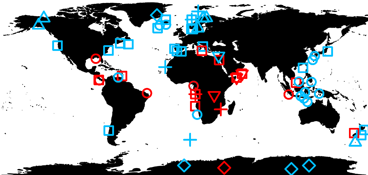
(a) M13
