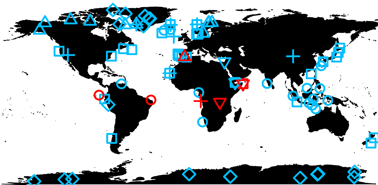
(c) R18
