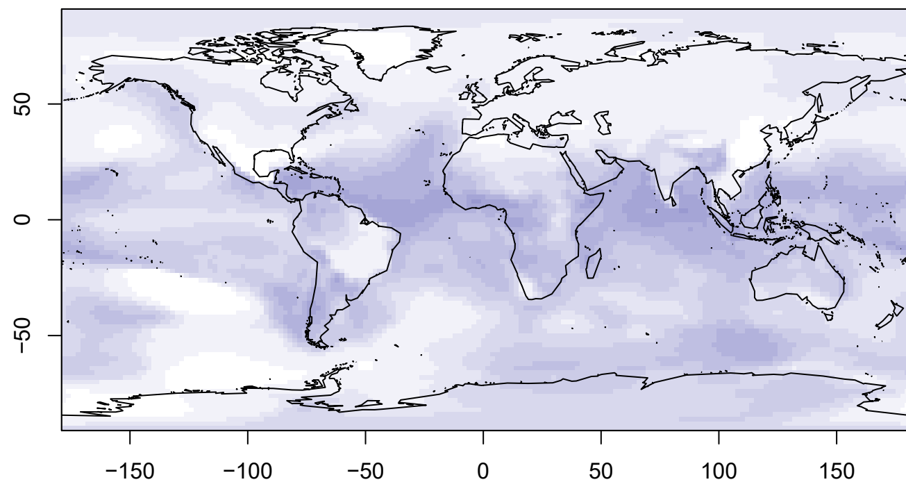
(f) Reanalysis (1871–1950)
