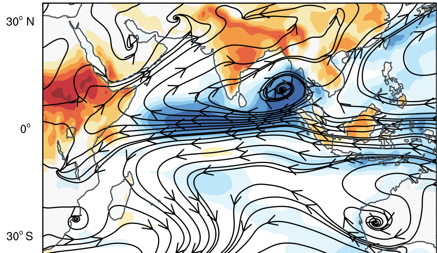
(b) P-E mm day -1
