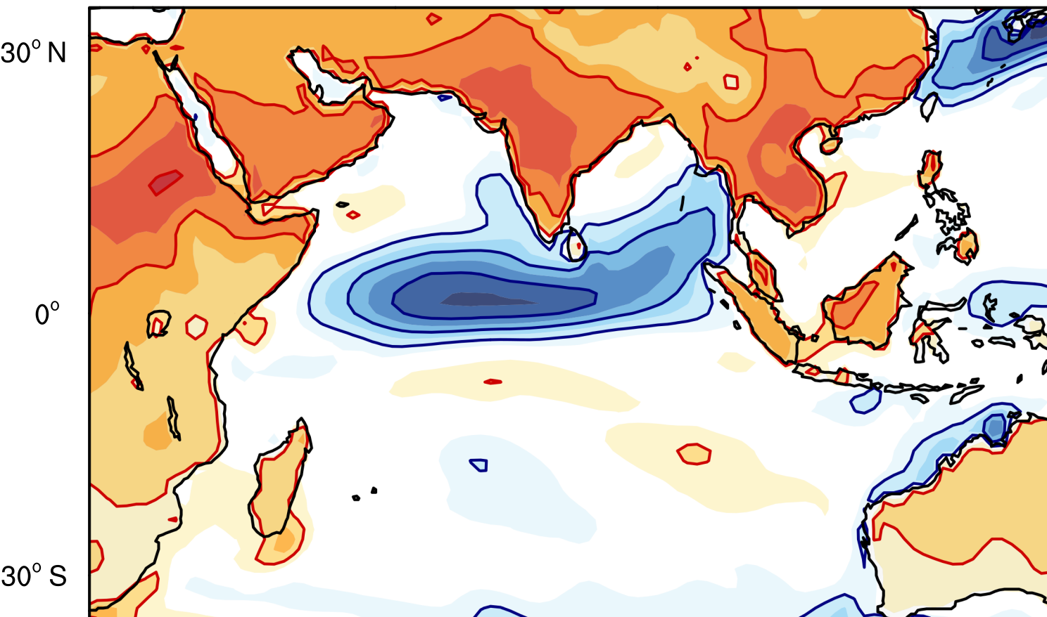
(a) Q_{div} mm day -1
