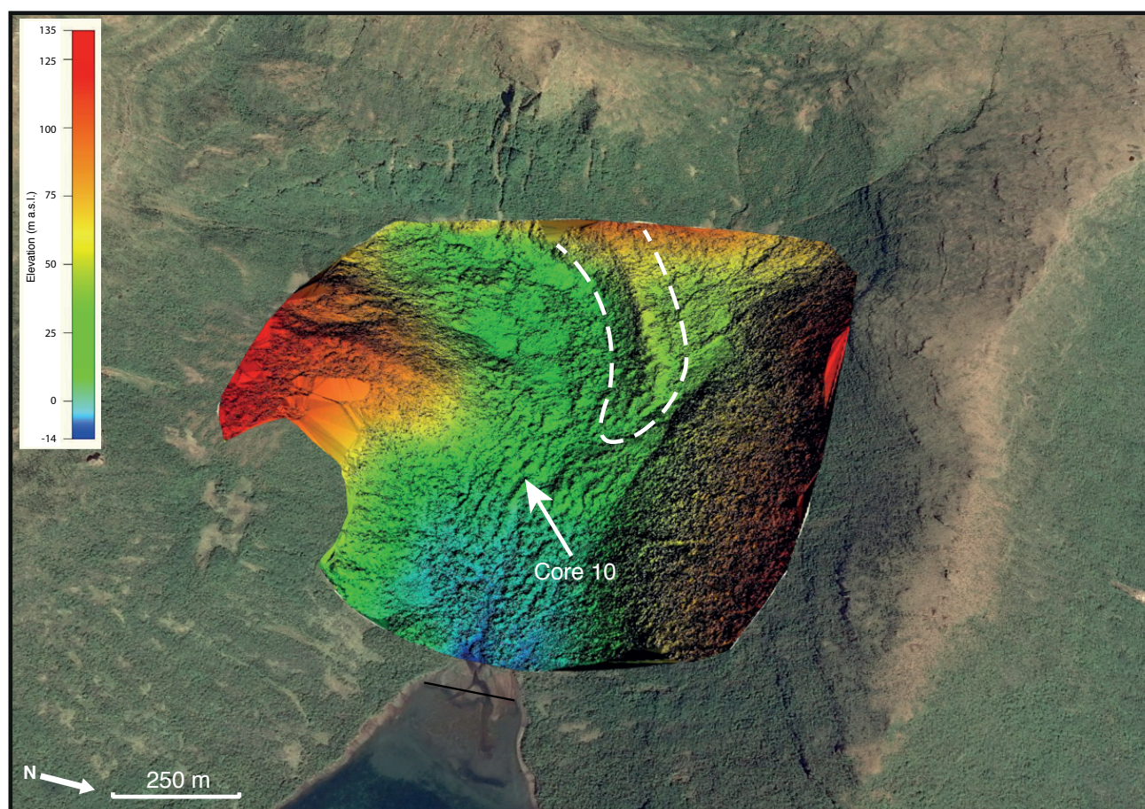
Supplementary Figure 1: Digital surface model of Musgrave Harbour, captured by Unmanned Aerial Vehicle and overlain on imagery from Google Earth, showing small cirques to the south-west and north-west. Lateral moraine between two cirque glaciers highlighted by white dashed lines. Location of Core 10 given by arrow.
