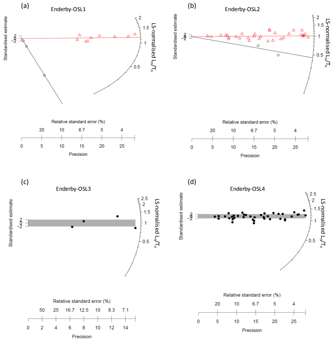
Supplementary Figure 6: Radial plots showing the LS-normalised L_n/T_n ratios for individual grains of each sample: (a) Enderby-OSL1, (b) Enderby-OSL2, (c) Enderby-OSL3 and (d) Enderby-OSL4. The red triangles and black circles in (a) and (b) distinguish the two components identified using the finite mixture model (FMM). The red and black lines are centred on the weighted mean values for each of these components, calculated using the FMM. The grey bands in (c) and (d) are centred on the weighted mean values estimated using the central age 5 model (CAM). The FMM and CAM were fitted to these data using the build-in functions in the R-package ‘Luminescence’ (Kreutzer et al., 2012).
