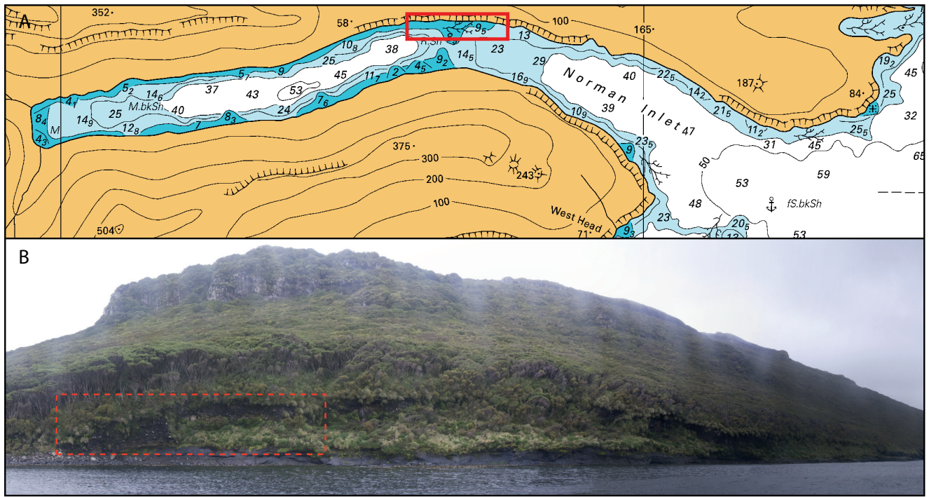
Supplementary Figure 9: (A) Hydrographic chart showing sill and over-deepening of Norman Inlet, east coast of Auckland Island (chart: NZ 2862, New Zealand Hydrographic Authority). Red box shows location of a potential moraine, shown in red dashed box in (B), taken on north shore of Norman Inlet (photo: Chris Turney).
