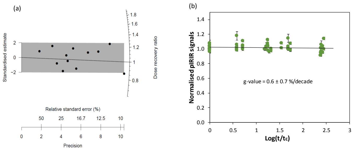
Supplementary Figure 4: (a) Radial plot (Galbraith et al., 1999; Galbraith and Roberts, 2012) of the dose recovery ratios (measured dose/given dose) for 12 accepted grains from Enderby-OSL1. The grey band is centred 5 on the weighted mean ratio (1.06) determined using the central age model. (b) Anomalous fading test on the pIRIR signals, made using 12 aliquots of K-feldspar from Enderby-OSL1.
