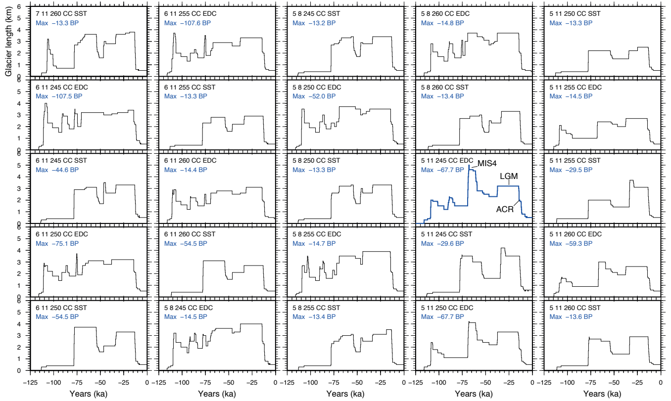
Supplementary Figure 10: Subset of the 25 simulations that have a MAAT of 5-7°C, constrained by realistic palaeo temperature reconstructions of the islands and which use a temperature-coupled precipitation regime. Plots show glacier length in km against time in ka. The simulation highlighted in blue is that which best fits all available field data (Figure 7A). MIS4, LGM and ACR are labelled.
