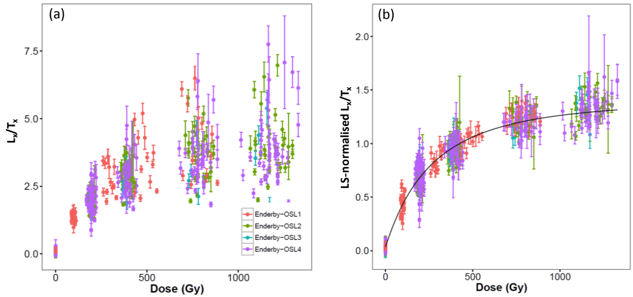
Supplementary Figure 5: (a) Sensitivity-corrected signals ( L_x/T_x ) for different grains of each of the Enderby samples. (b) LS-renormalised L_x/T_x ratios, using the same data as shown in (a). LS-normalisation was achieved using the built-in function provided in the R-package ‘numOSL’ (Peng et al., 2013; Peng and Li, 2017). The 5 black line is the best-fit curve obtained using the general-order kinetic model (Guralnik et al., 2015).
