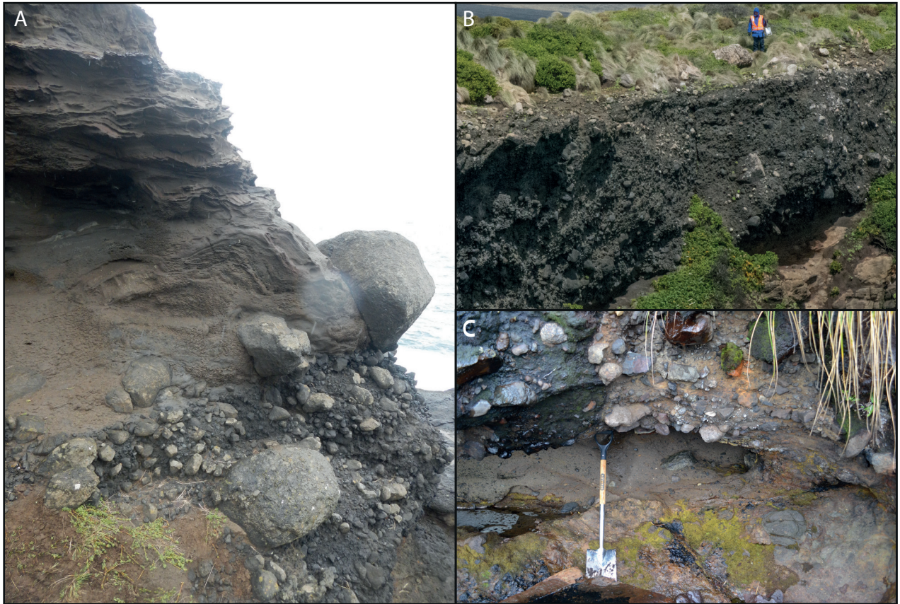
Supplementary Figure 8: Photos showing details of glacial ‘Enderby Till’ at (A) Enderby Formation, (B) Pillar Rock, (C) Emergency Bay.
