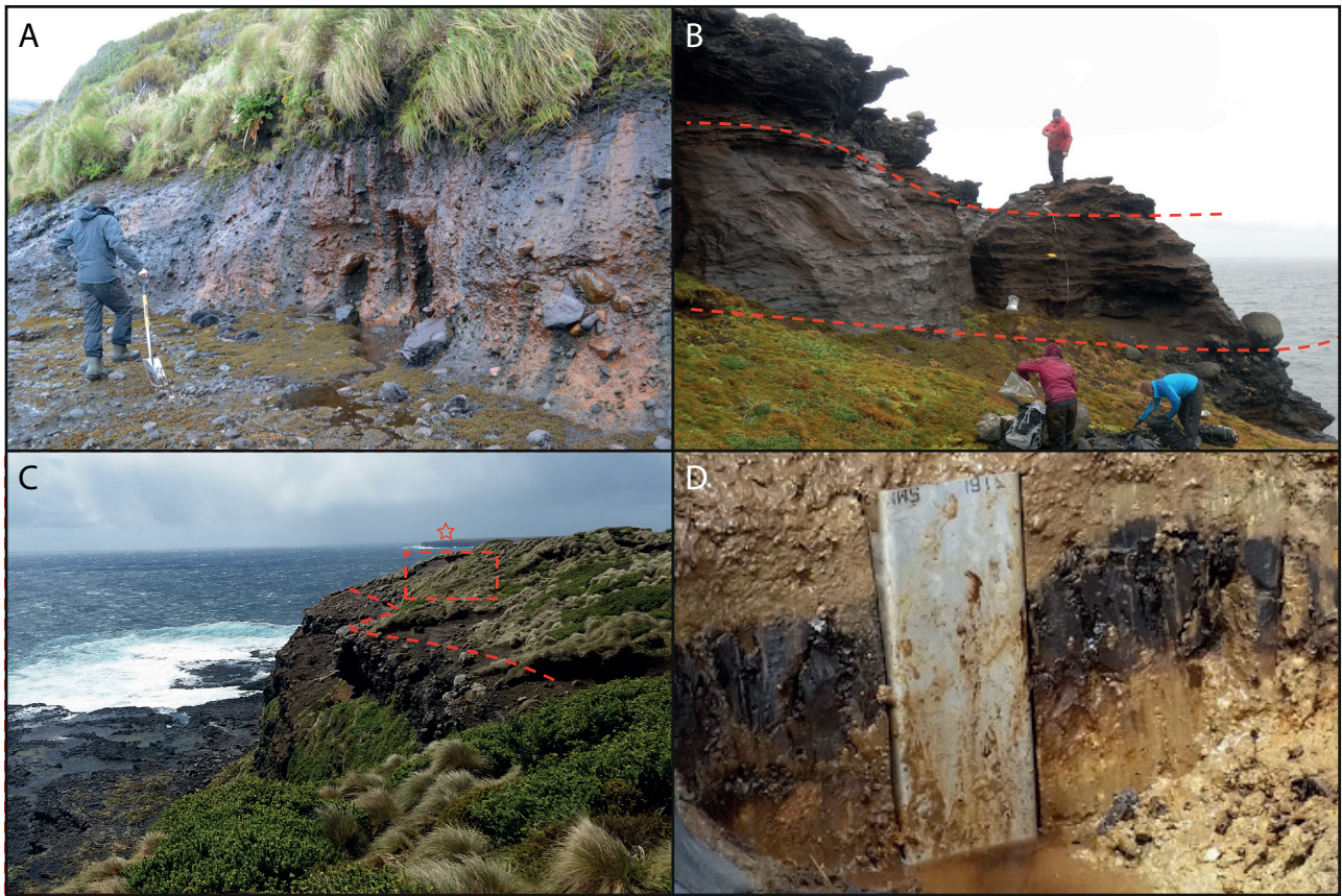
Supplementary Figure 7: Photos showing sediment deposits at (A) Emergency Bay (photo: Verity Flett), (B) Enderby Island (photo: Greg de Wet) and (C) Pillar Rock (photo: Chris Turney). Red dashed lines in (B) show delineation of upper and lower tills, with laminated lake sediments in between. Red box in (C) shows location of Pillar Rock Formation, red dashed line delineates upper boundary of glacial till, red star shows location of Enderby Island (just visible on horizon) in relation to the Pillar Rock formation. (D) shows organic silts from 237-250 cm in the Pillar Rock sediment sequence (photo: Chris Turney).
