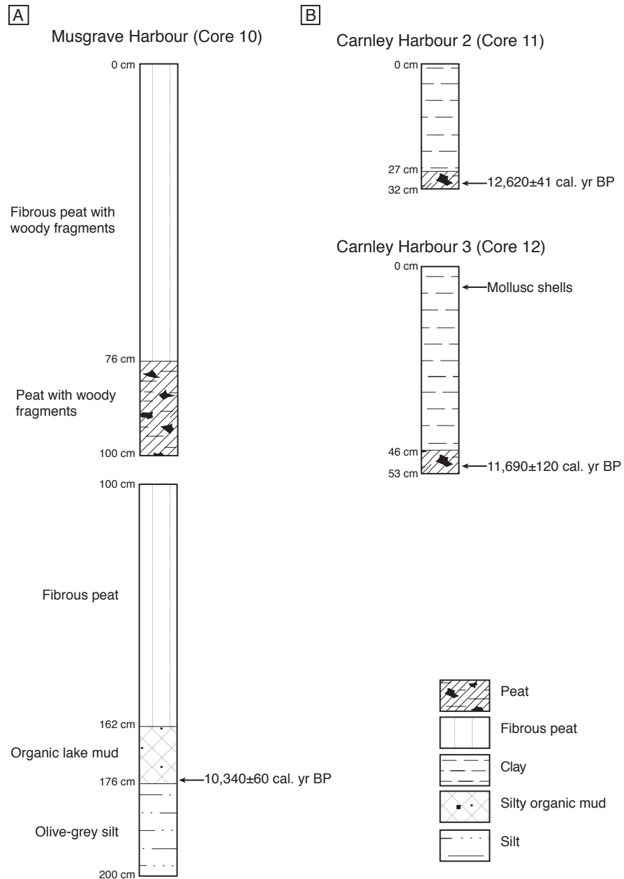
Supplementary Figure 2: Schematics of sediment cores. (A) Core taken from Musgrave Harbour (Core 10). (B) Two marine cores from Carnley Harbour (Cores 11 and 12).
