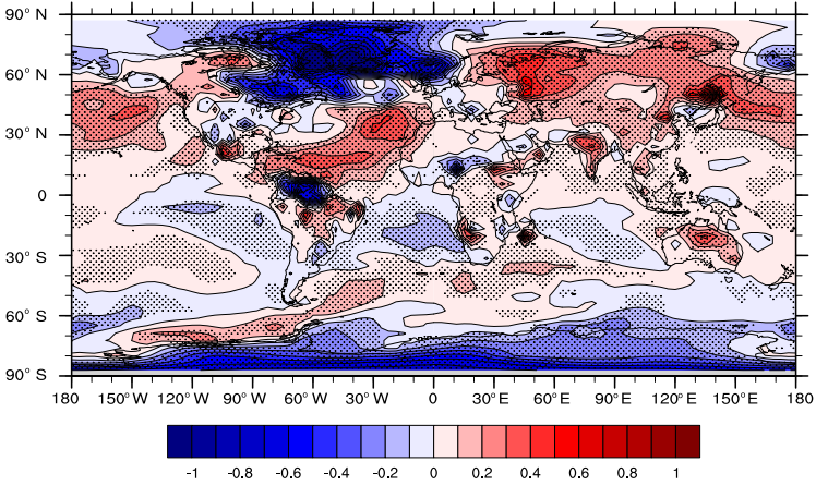
(a) Temperature
