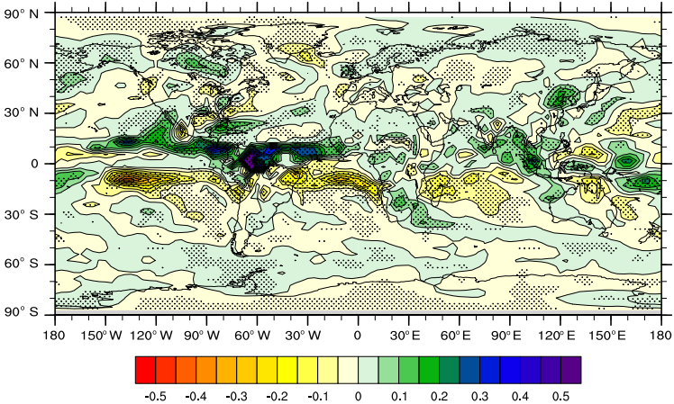
(b) Precipitation
