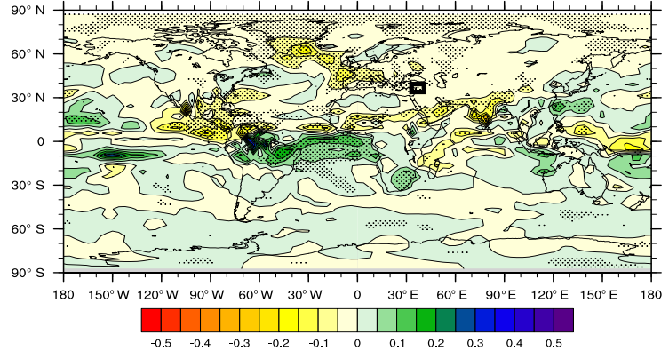
(b) Precipitation
