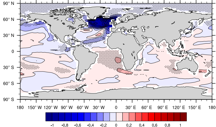
(c) SST
