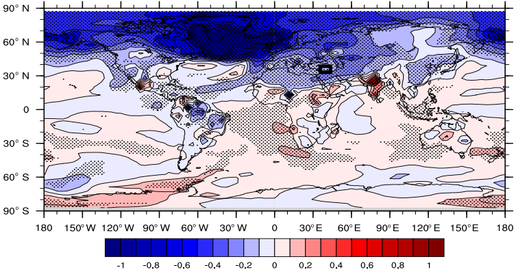
(a) Temperature
