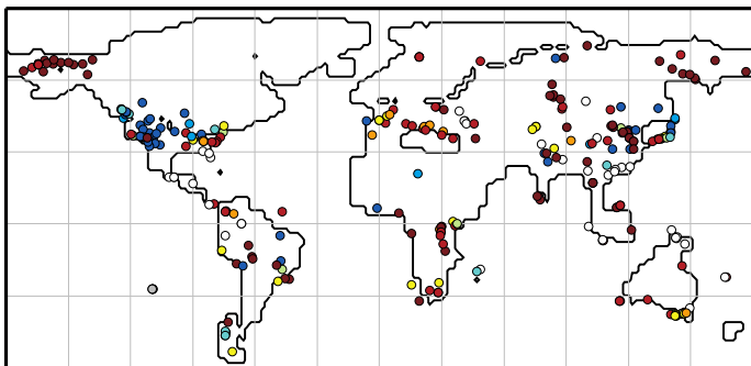
BNS for FPC method vs. records LGM
