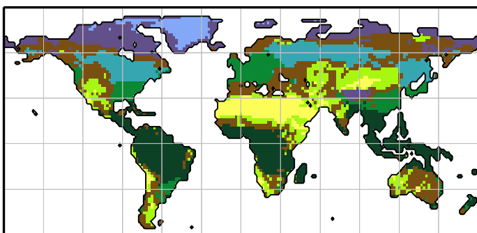
FPC method LGM
