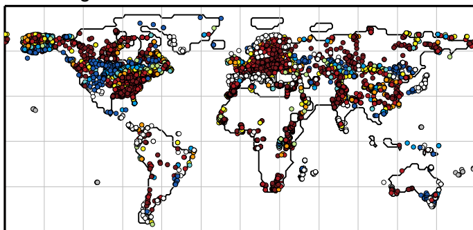
BNS for PFT method vs. records LGM
