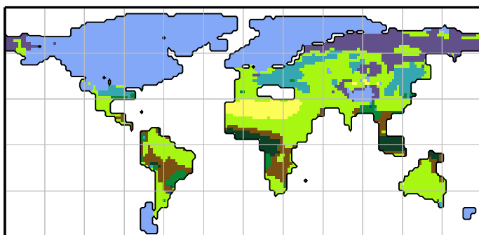
PFT method LGM
