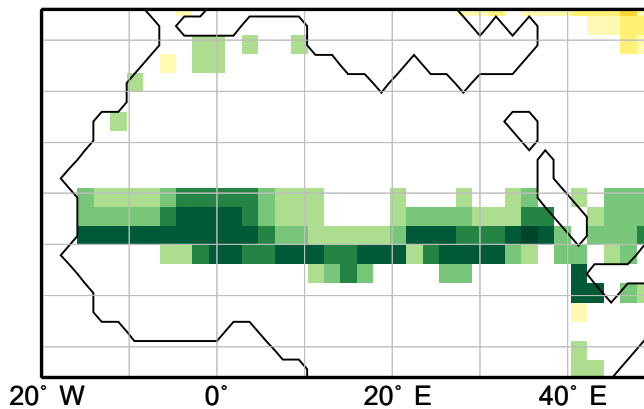
CLIM-LPJ
