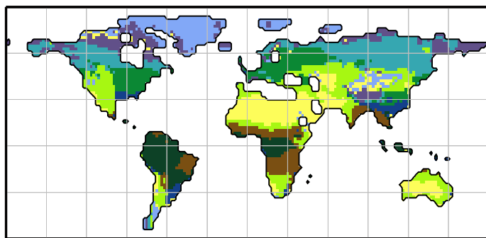
CLIM-LPJ
