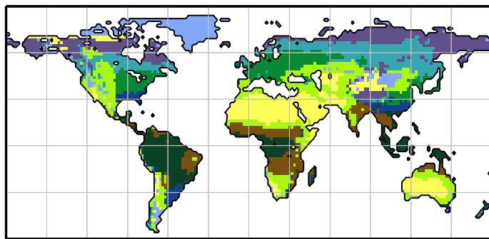
CLIMBER-VECODE
