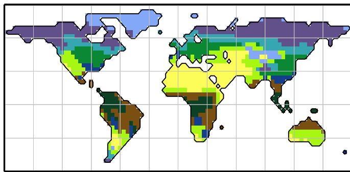
IPSL-ESM-T63
