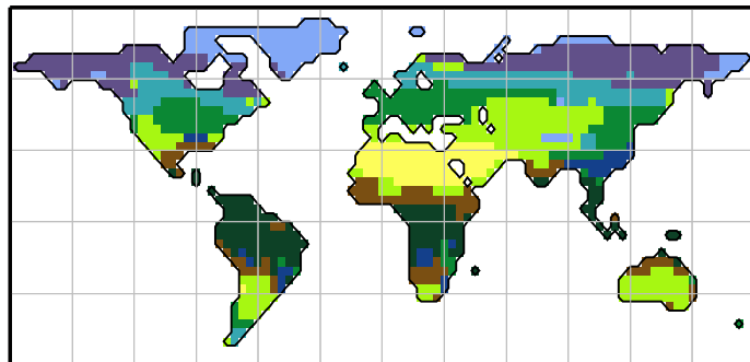
IPSL-ESM-T63
