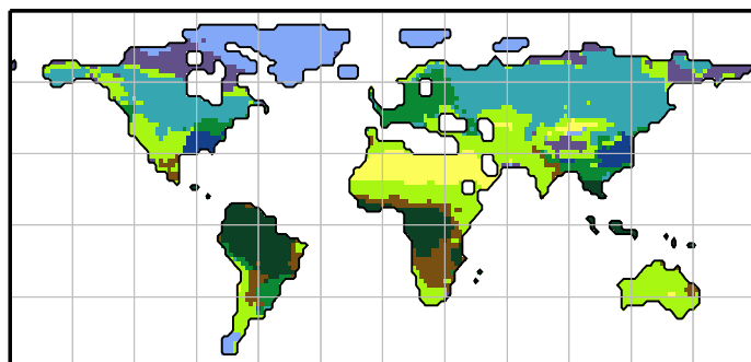
CLIM-LPJ
