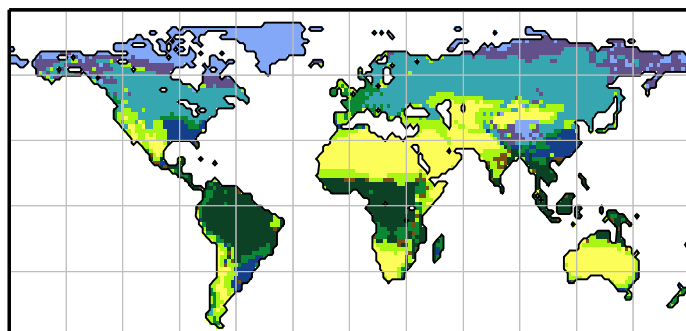
CLIMBER-VECODE
