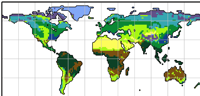
IPSL-ESM-T31
