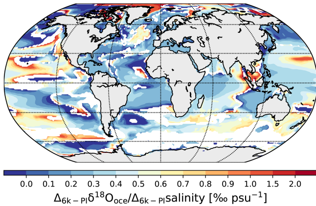
Figure 13. Spatial distribution of calculated temporal 6k-PI \delta^{18}\text{O}_{\text{occe}} -salinity gradients for oceanic grid cells in which the 6k-PI absolute change in salinity is at least 0.02 psu.
