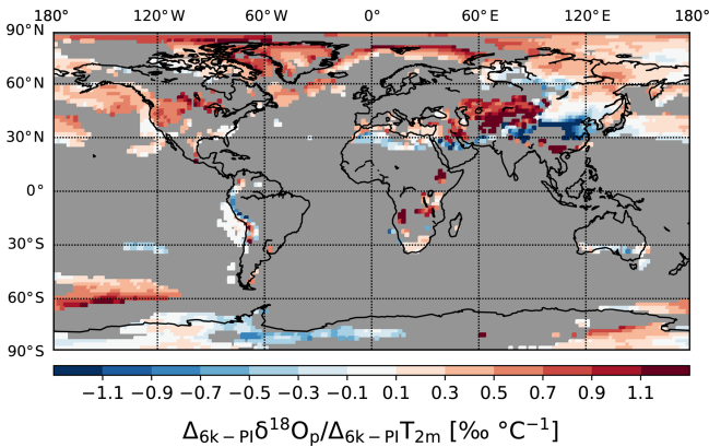
Figure 11. Spatial distribution of the calculated temporal 6k-PI \delta^{18}O_p - T gradients for all grid cells in which (i) simulated annual mean temperature for both PI and 6k is lower than 20°C and (ii) absolute change in temperature between the 6k and PI control simulations is at least 0.5°C. The gradients are calculated in the same way as in Fig. 10b but with the use of precipitation-weighted temperatures instead of arithmetic annual mean temperatures.
