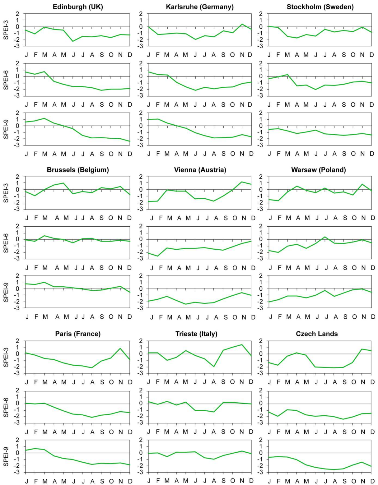
Figure S3. Annual variation of SPEI-3, SPEI-6 and SPEI-9 for selected European stations and regions in 1842
