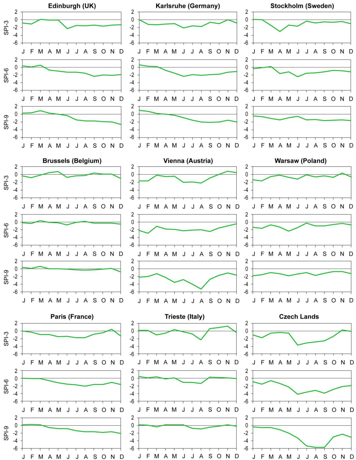
Figure S2. Annual variation of SPI-3, SPI-6 and SPI-9 for selected European stations and regions in 1842
