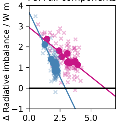
TOA all components
