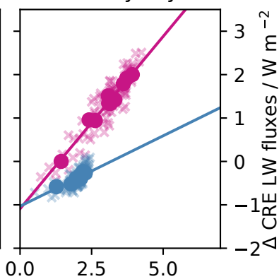
TOA cloudy-sky LW
