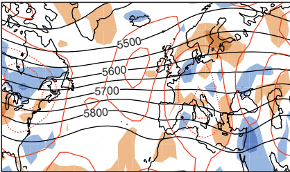
(a) 1847–1876 minus 30 yr before and after
