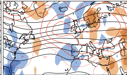
(b) 1943–1972 minus 30 yr before and after
