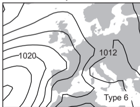
N cyclonic
