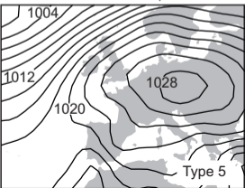
HP over Europe
