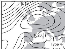
E indifferent
