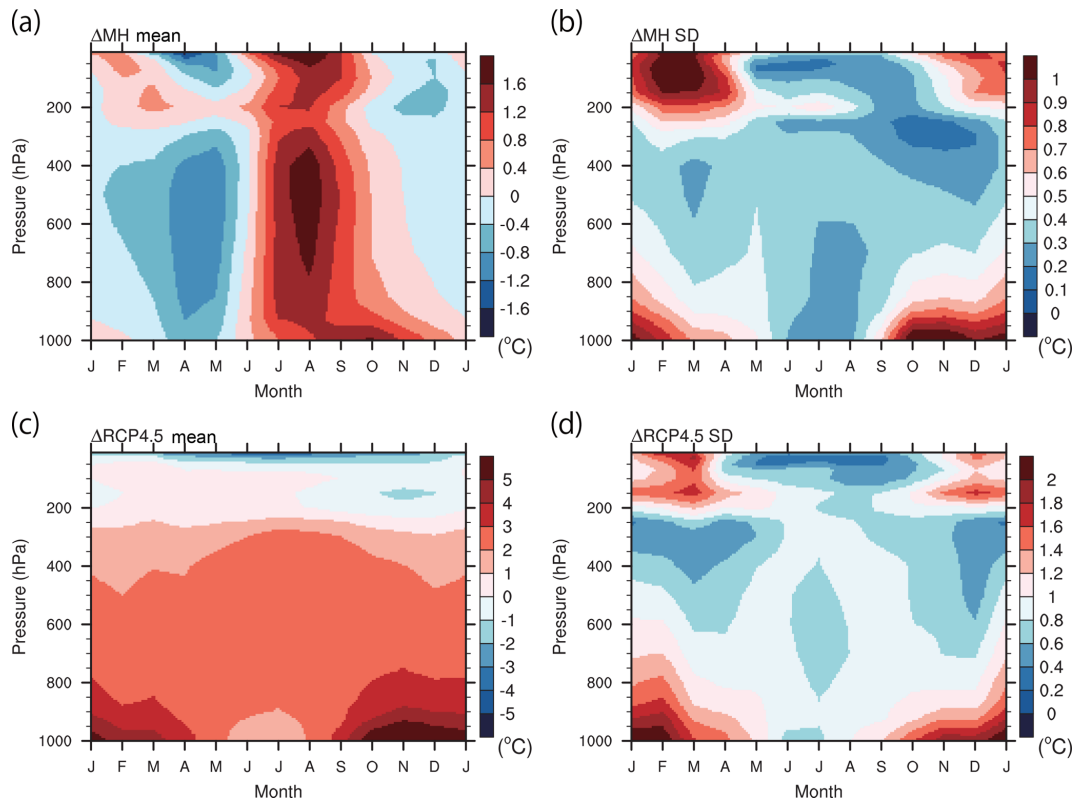
Figure 7. Same as in Fig. 6 but for the air temperature change (°C) (north of 60° N). All 10 models listed in Table 2 are used. (Note that the figure appears blocky compared to Fig. 6 due to the use of a different interpolation scheme in the plotting software which was chosen to avoid a technical issue for pressure coordinate, but it is irrelevant to the data.)
