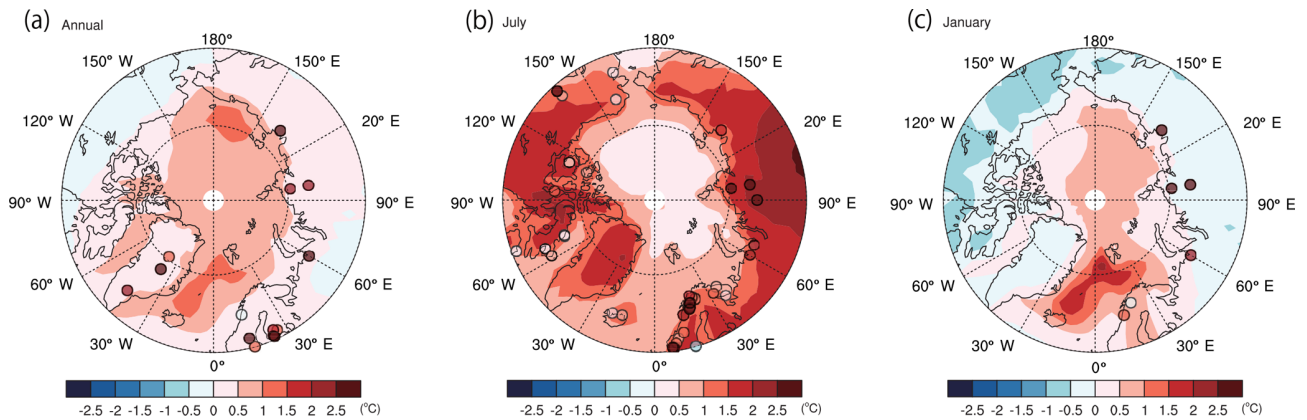
Figure 4. Surface air temperature anomaly ( ^{\circ}\text{C} ) for \Delta\text{MH} from the simulations (shading) and reconstruction (solid circles): (a) annual mean; (b) July; and (c) January. The reconstruction data are taken from Sundqvist et al. (2010). The mean of all 10 models listed in Table 2 was used.
