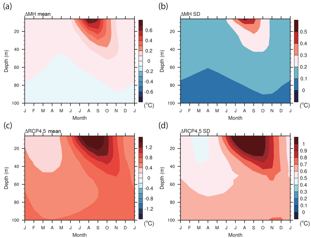
Figure 10. Same as in Fig. 6 but for the upper ocean temperature change ( ^{\circ}\text{C} ) (north of 60^{\circ}\text{N} ). The nine models except for FGOALS-g2 listed in Table 2 are used.
