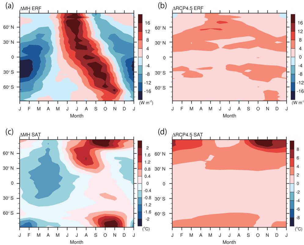
Figure 2. Seasonal progress of the zonal mean effective radiative forcing, effective radiative forcing (ERF) ( a , b ; \text{W m}^{-2} ), and surface air temperature change ( c , d , ^{\circ}\text{C} ): ( a , c ) \Delta\text{MH} and ( b , d ) \Delta\text{RCP4.5} . The ERF for \Delta\text{RCP4.5} is drawn using the data from Yoshimori et al. (2018), and it is computed in the current study for \Delta\text{MH} . Both ERFs are constructed with a single model, MIROC4m-AGCM (Yoshimori et al., 2018). The surface air temperature changes are the means of all 10 models listed in Table 2.
