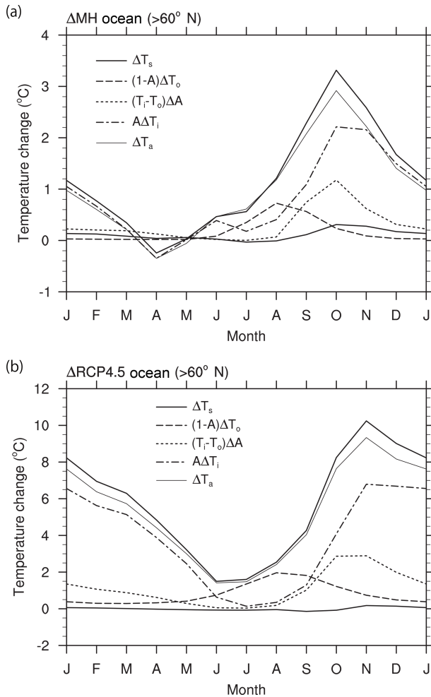
Figure 9. Contribution of the individual components to the surface temperature change ( ^{\circ}\text{C} ) over the ocean (north of 60^{\circ}\text{N} ): (a) \Delta\text{MH} and (b) \Delta\text{RCP4.5} . The surface temperature change is decomposed into the components of the SST change ( (1-A)\Delta T_o ), sea ice concentration change ( (T_i - T_o)\Delta A ), and sea ice surface temperature change ( A\Delta T_i ). Simulated surface temperature ( \Delta T_s ) and surface air temperature changes ( \Delta T_a ) are also plotted for reference. Only five models (bcc-csm-1, CCSM4, CNRM-CM5, IPSL-CM5A-LR, and MRI-CGCM3) are used.
