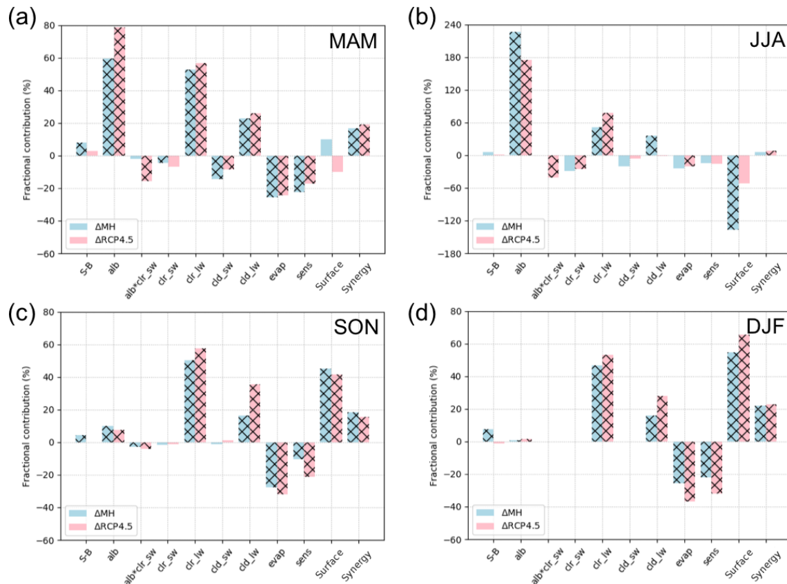
Figure 12. Fractional contribution of individual processes to the model spread in the simulated surface temperature change (%) over the ocean (north of 60^{\circ} N) for \Delta MH and \Delta RCP4.5: (a) spring (March–April–May); (b) summer (June–July–August); (c) autumn (September–October–November); and (d) winter (December–January–February) means. The sum of the bar graphs in the same color for each plot adds up to 100%. The hatching indicates the contribution is statistically significant at the 10% level. All 10 models listed in Table 2 are used. See Table 3 for the interpretation of each component. Note that the vertical scale for panel (b) is 3-fold larger than those for the other plots.
