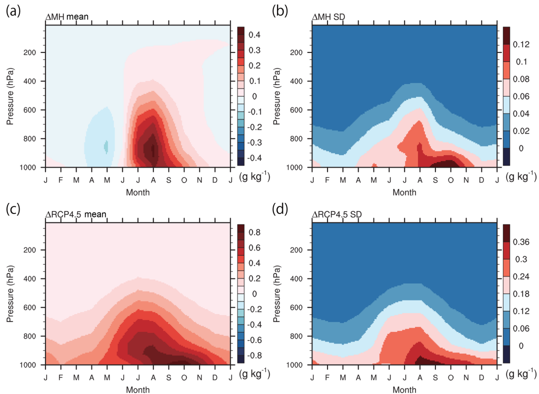
Figure 8. Same as in Fig. 6 but for the specific humidity change ( \text{g kg}^{-1} ) (north of 60^\circ \text{N} ). All 10 models listed in Table 2 are used. (Note that the figure appears blocky compared to Fig. 6 due to the use of a different interpolation scheme in the plotting software which was chosen to avoid a technical issue for pressure coordinate, but it is irrelevant to the data.)
