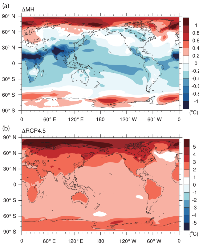
Figure 1. Multi-model mean (all 10 models listed in Table 2) annual mean surface air temperature response (°C): (a) \Delta\text{MH} and (b) \Delta\text{RCP4.5} .
