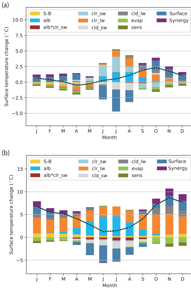
Figure 5. Simulated and diagnosed surface temperature changes ( ^{\circ}\text{C} ) for the ocean (north of 60^{\circ}\text{N} ): (a) \Delta\text{MH} and (b) \Delta\text{RCP4.5} . The solid black polygonal lines denote simulated changes and dashed blue polygonal lines denote the sum of the diagnosed partial changes; the two lines are superimposed. The graphs represent the means of all 10 models listed in Table 2. See Table 3 for the interpretation of each component.
