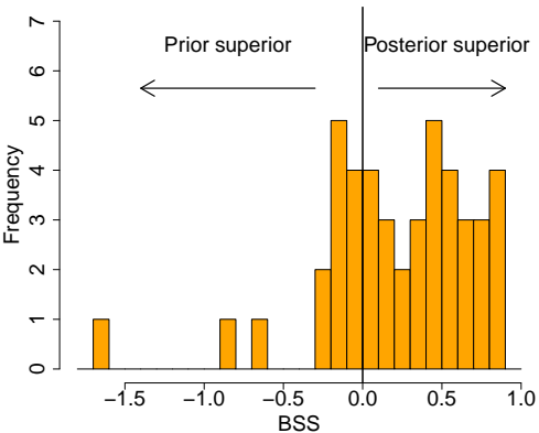
(a) Cross-validation: histogram of BSS
