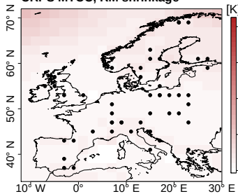
CRPS MTCO, RM shrinkage
