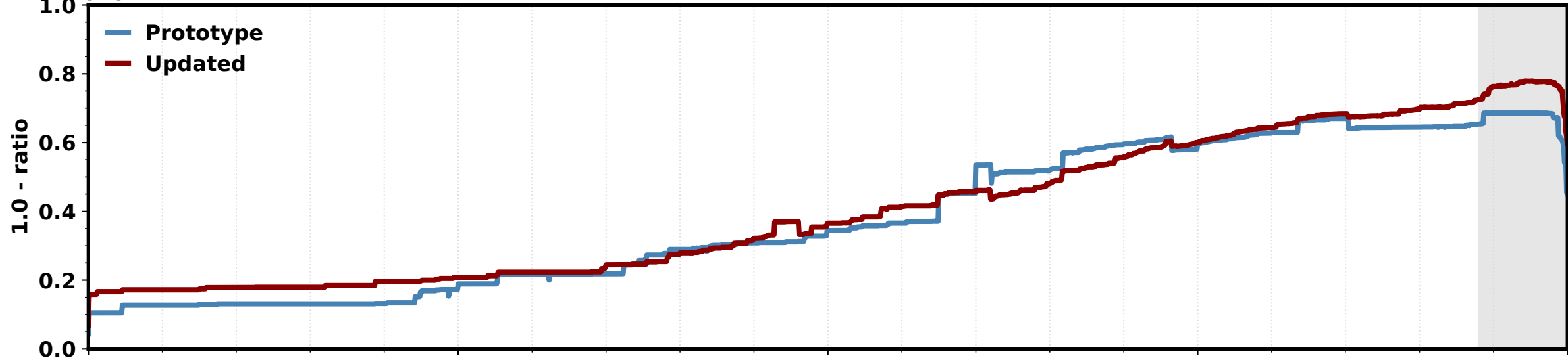
(c) NH mean temperature
