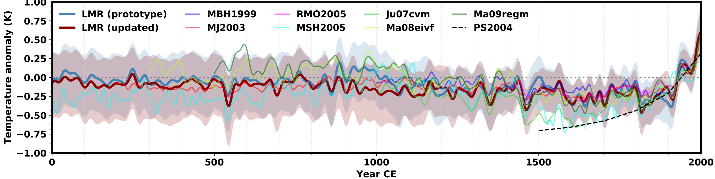
(c) NH mean temperature
